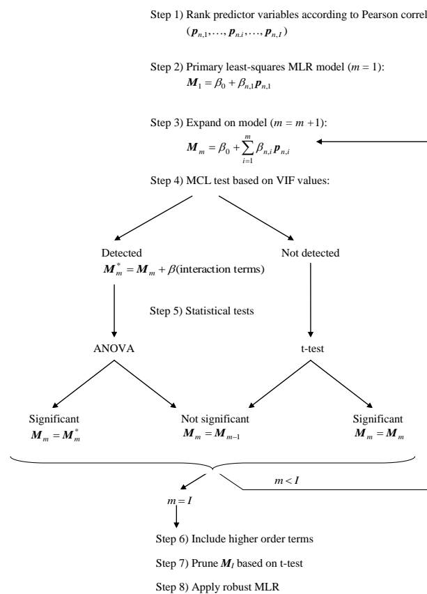
Fig. 2. Schematic diagram of our robust forward MLR routine.
