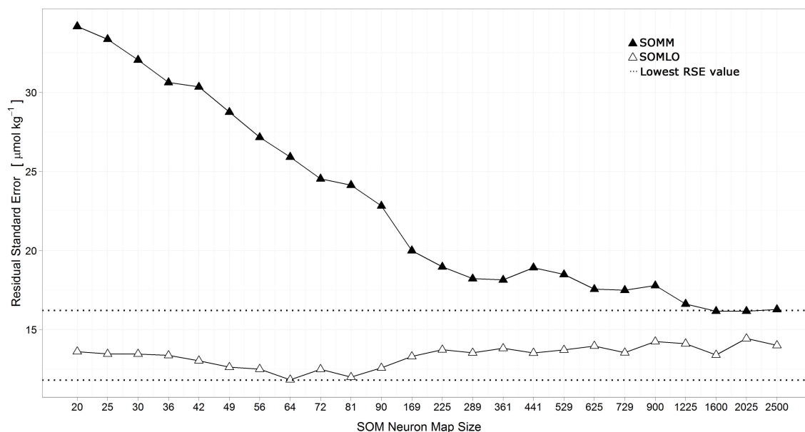
Fig. 10. Skill comparison between the SOMLO and SOMM models in capturing C_T .
