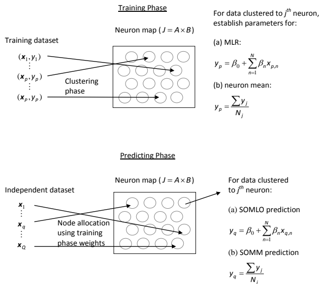
Fig. 4. Schematic diagram of neural network training and prediction phases.
