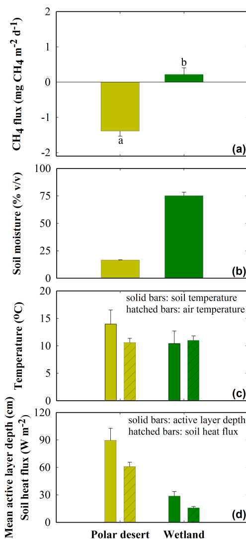
Figure 3. Comparison of 2010–2012 growing season mean \text{CH}_4 fluxes ( F_{\text{CH}_4} ; \pm 1\text{SE} ) measured in chambers (a) and other environmental variables (b–d), paired by site. The sampling period represented by each bar spans approximately late June to early August. Letters indicate if there were statistically significant differences of F_{\text{CH}_4} between sites using a repeated-measures ANOVA.
