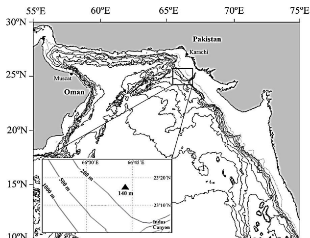
Figure 1. Location of the study site at 140 m water depth on the Pakistan margin of the Indian Ocean.
