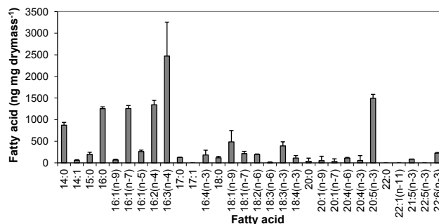
Figure 2. Quantity ( \text{ng mg dry mass}^{-1} ) of fatty acids in the ^{13}\text{C} -labelled diatom, Thalassiosira weissflogii ( n = 2 replicate samples).
