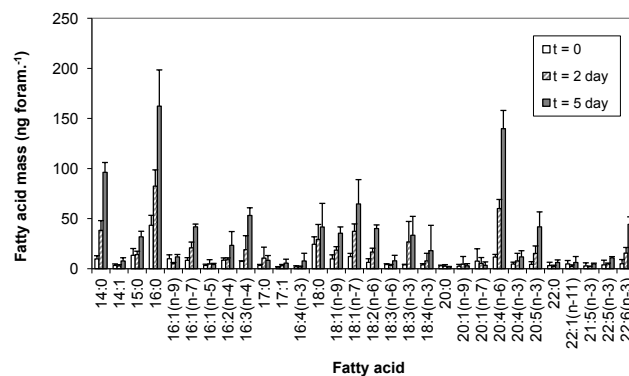
Figure 5. Changes in the amounts of fatty acids ( \text{ng foram}^{-1} ) in Uvigerina ex. gr. semiornata during the shipboard experiment ( n = 4 replicate samples of 30 foraminifera). 95 % confidence intervals are indicated.
