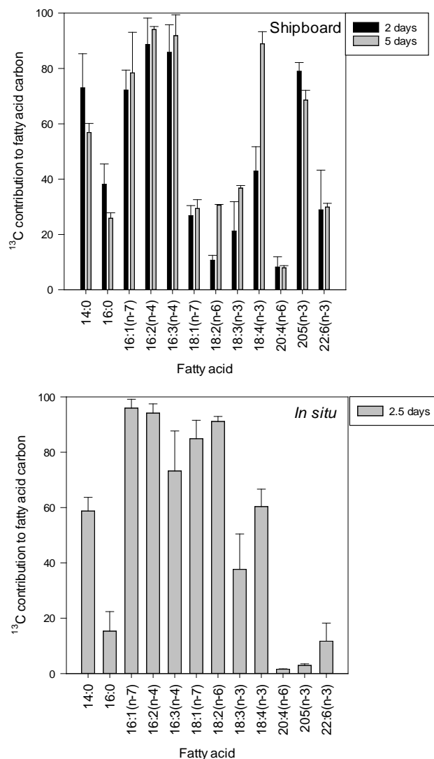
Figure 7. Percentage ^{13}\text{C} labelling of twelve dominant fatty acids in Uvigerina ex. gr. semiornata during shipboard (upper panel) and in situ (lower panel) incubations. Data are average values of 4 replicate samples (each of 30 foraminifera). 95 % confidence intervals are indicated for ^{13}\text{C} values
