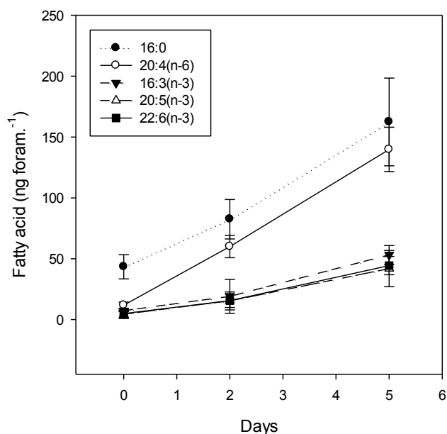
Figure 6. Increase in amounts of five key fatty acids in Uvigerina ex. gr. semiornata during the shipboard experiment (control samples, 2-day and 5-day incubations). 95 % confidence intervals are indicated.
