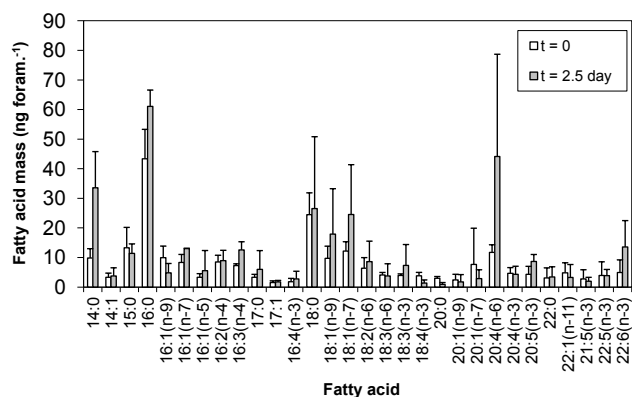
Figure 4. Changes in the amounts of fatty acids ( \text{ng foram}^{-1} ) in Uvigerina ex. gr. semiornata during the in situ experiment ( n = 4 replicate samples of 30 foraminifera). 95 % confidence intervals are indicated.
