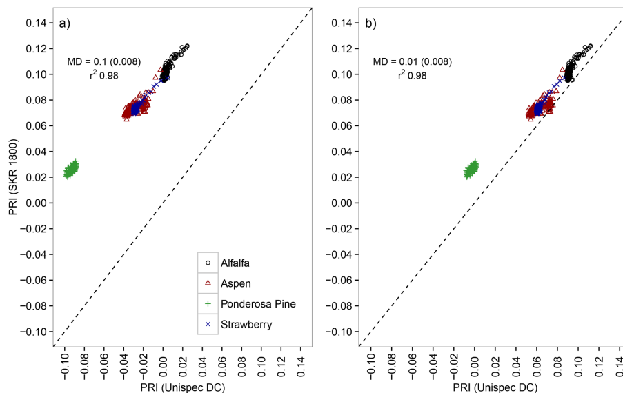
Figure 3. Scatter plots of UniSpec DC photochemical reflectance index (PRI) vs. SKR 1800 PRI across a range of plant canopies during a series of dark-to-light transitions. (a) Depicts the data without correction for differences in SRFs and (b) depicts the data after normalization for differences in the spectral configuration. The dotted lines represent the 1 : 1 line. MD in the plots stands for mean differences and the values in the parentheses are the standard deviation of the differences.
