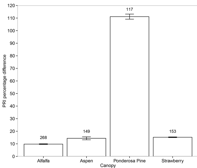
Figure 4. Plant canopy dependencies of UniSpec DC photochemical reflectance index (PRI) vs. SKR 1800 PRI across a range of plant canopies during a series of dark-to-light transitions. Per-canopy mean percentage differences are plotted along with 95 % confidence intervals. The sample sizes (number of pairs) used to compute the mean differences and confidence intervals are given at the tops of the bars. Data shown are those that have been corrected to normalize the SRF differences between instruments.
