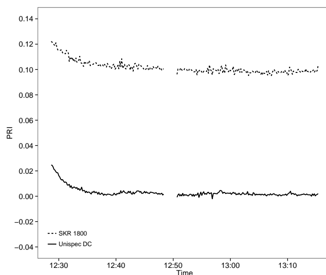
Figure 2. Photochemical reflectance index (PRI) response to a dark-to-light transition for alfalfa ( Medicago sativa ), as recorded by a UniSpec DC instrument and the SKR 1800 sensor pair.
