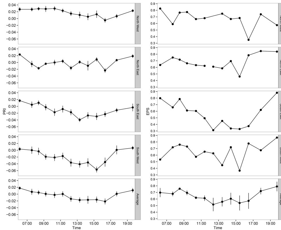
Figure 9. Diurnal course of lodgepole pine ( Pinus contorta ) leaf-level photochemical reflectance index (PRI) and the epoxidation state of the xanthophyll cycle components (EPS). PRI values for each of the four directions are means of 10 sampled spectra. Error bars represent \pm 1 standard error of mean.
