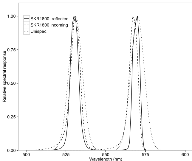
Figure 1. Spectral response curves for the UniSpec instruments and the upward- (incoming) and downward-looking (reflected) SKR 1800 sensor pair.
