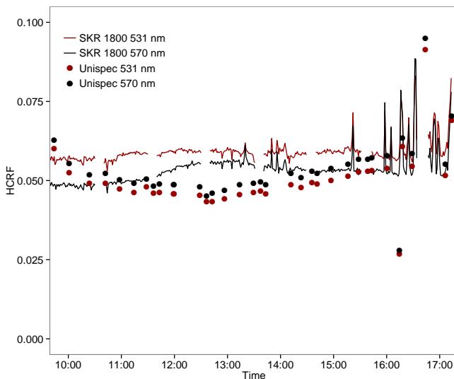
Figure 8. Hemispherical–conical reflectance factors (HCRFs) at 531 and 570 nm obtained by a UniSpec and SKR 1800 sensor pair, as a function of time of day. Data were collected over a lodgepole pine ( Pinus contorta ) canopy and corrected to reflectance using cross-calibration functions determined from white panel measurements. Only data that were collected within the time frame of white panel measurements are shown. Data shown have not been normalized to correct for the SRF differences between instruments.
