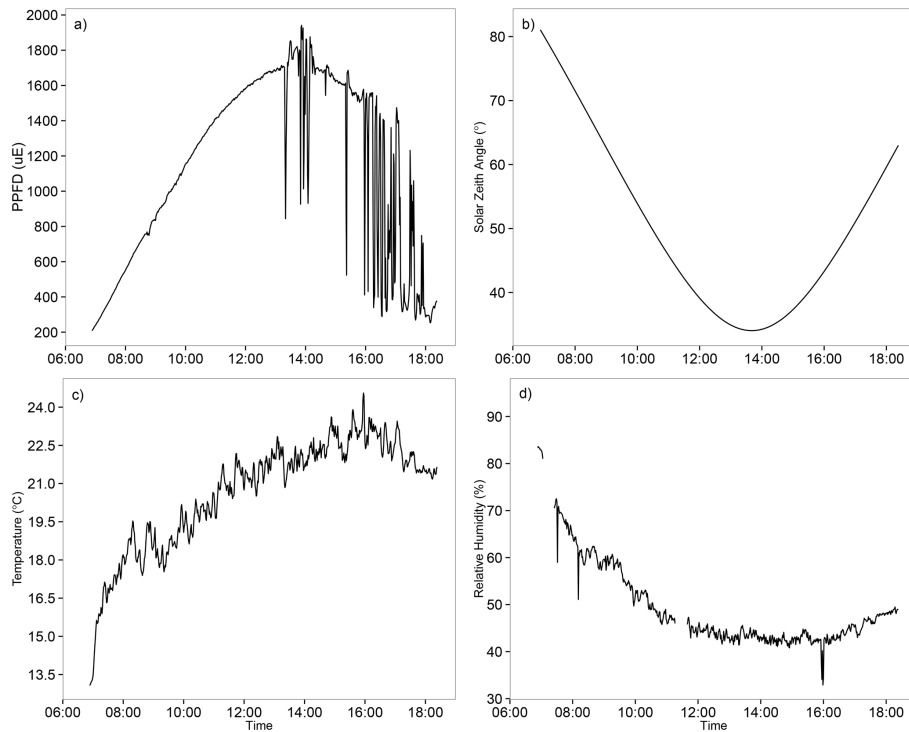
Figure 6. (a) Photosynthetic photon flux density (PPFD), (b) solar zenith angle (SZA), (c) temperature and (d) relative humidity as a function of time of day (July 25, 2013).
