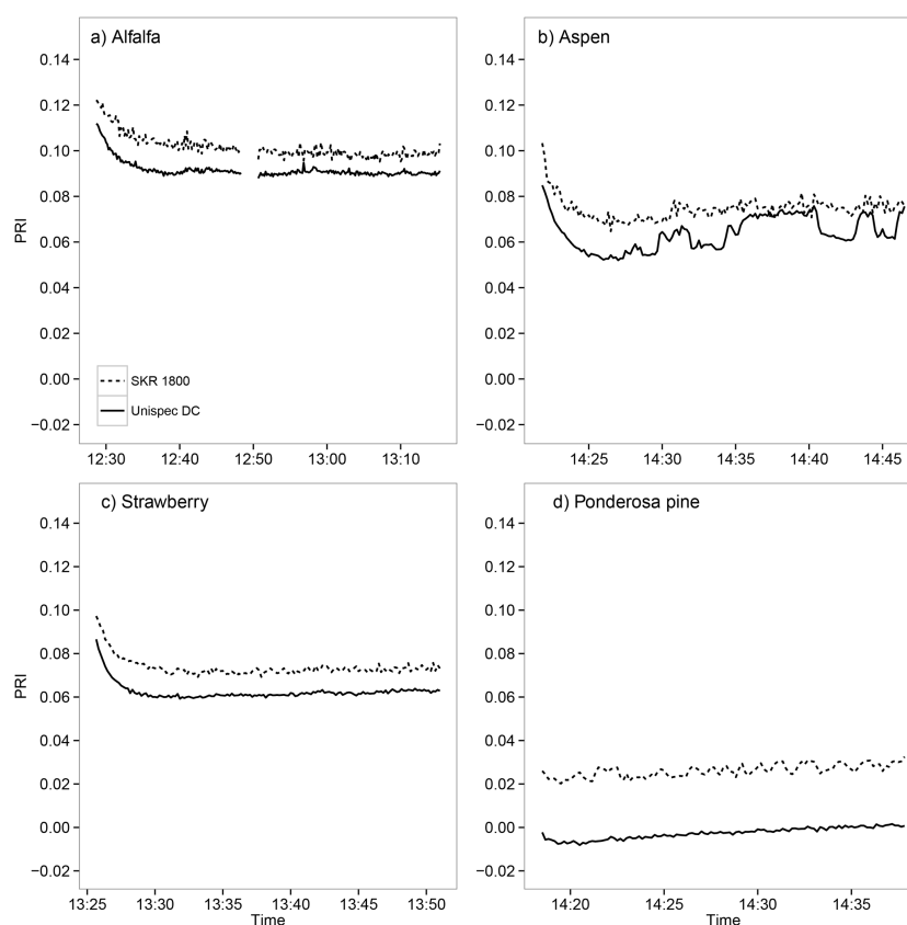
Figure 5. Photochemical reflectance index (PRI) response to a dark-to-light transition for (a) alfalfa ( Medicago sativa ), (b) aspen ( Populus tremuloides ), (c) strawberry ( Fragaria × ananassa ), and (d) ponderosa pine ( Pinus ponderosa ), as recorded by a UniSpec DC instrument and the SKR 1800 sensor pair. Data shown are those that have been corrected to normalize the SRF differences between instruments.
