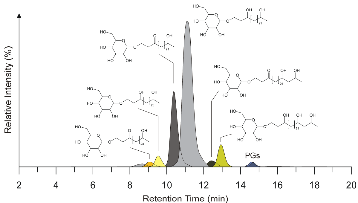
Fig. S1. Composite HPLC/MS chromatogram showing the distribution of heterocyst glycolipids in a water column filtrate of Lake Schreventeich collected in early September. Note that mass traces of the HG 26 diol and HG 26 keto-ol contained additional signals at around 14.7 min, which resulted from the in-source fragmentation of phosphatidylglycerols (PGs).
