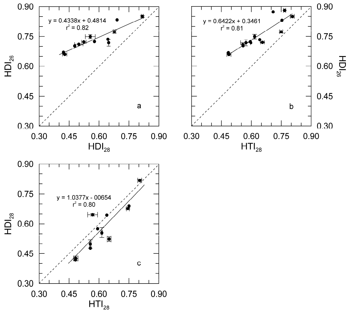
Figure S3. Correlations between the different HG indices determined in this study. (a) HDI 26 vs. HDI 28 , (b) HDI 26 vs. HTI 28 and (c) HDI 28 vs. HTI 28 . Dashed lines represent 1:1 lines. Note that all correlations are statistically significant with p -values < 0.001 .
