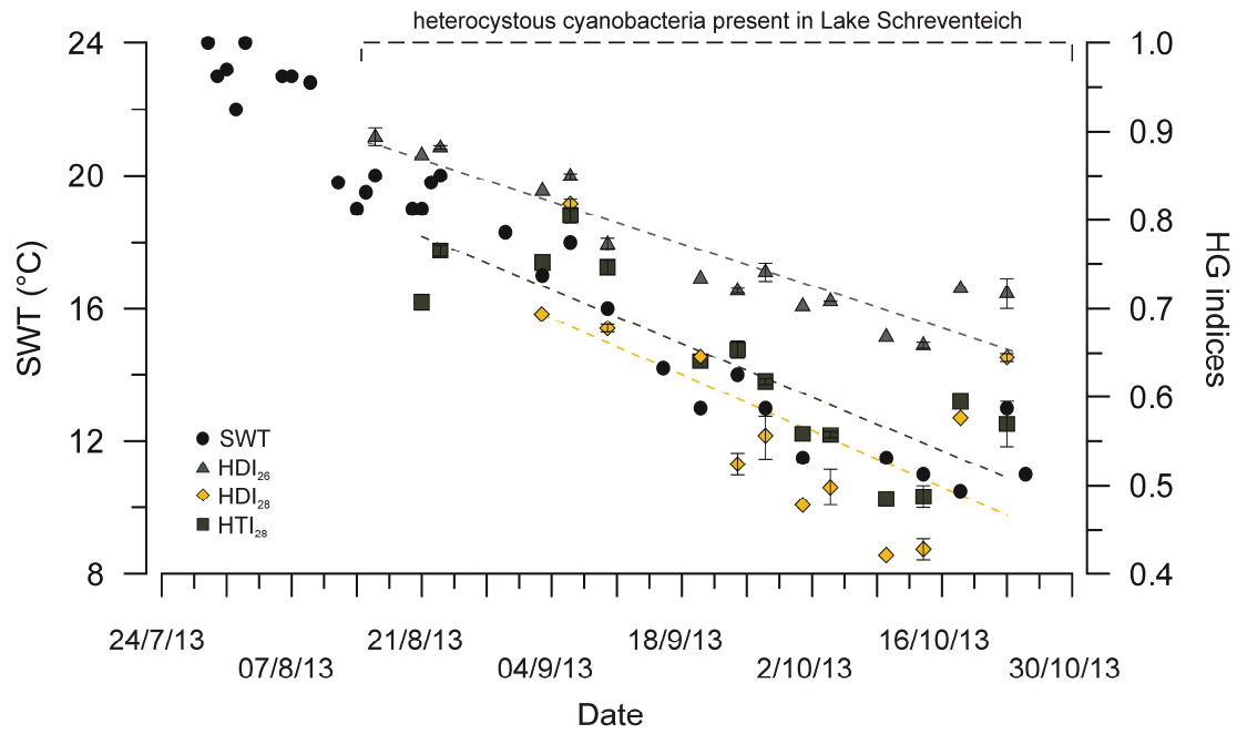
Figure S2. Comparison of measured surface water temperatures (SWT) with variation of calculated HG indices (e.g. HDI 26 , HDI 28 and HTI 28 ) in Lake Schreventeich over time.
