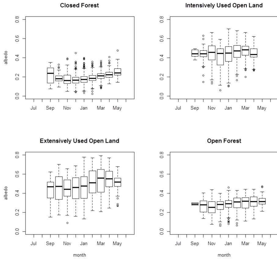
Figure A3. Seasonal variation of the albedo values of the four snow-covered LULC classes: closed forest, intensively used open land, extensively used open land and open forest (full BRDF albedo values and magnitude inversion albedo values for open forest).
