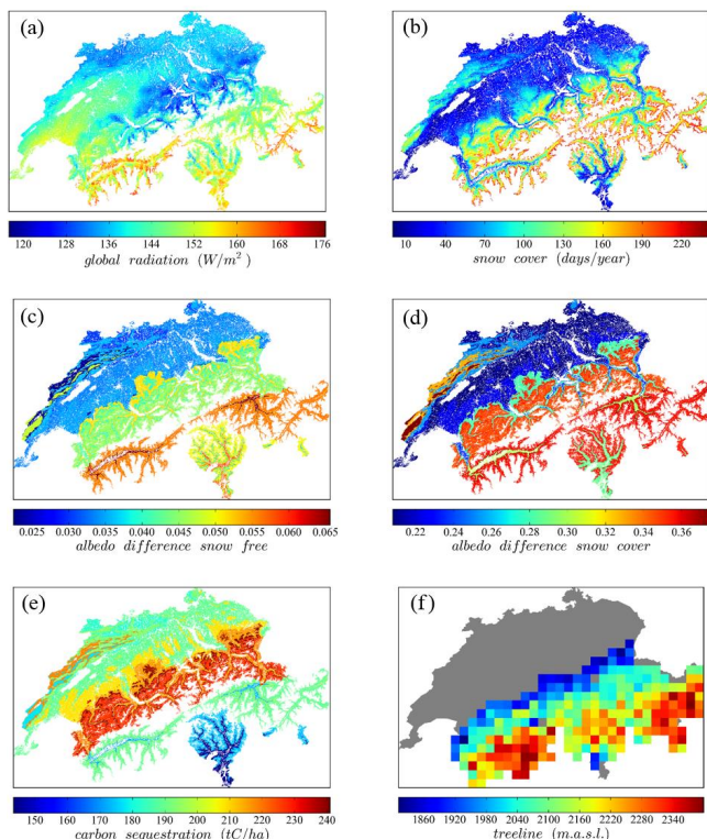
Figure 3. (a) Mean yearly global radiation. (b) Days with snow cover per year. (c) Albedo difference without snow (difference between intensively and extensively used open land and closed forest). (d) Albedo difference with snow (difference between intensively and extensively used open land and closed forest). (e) Carbon sequestration (difference between intensively and extensively used open land and closed forest). (f) Treeline elevation calculated using the Swiss area statistics of 1997 and applying the method of Paulsen and Körner (2001).
