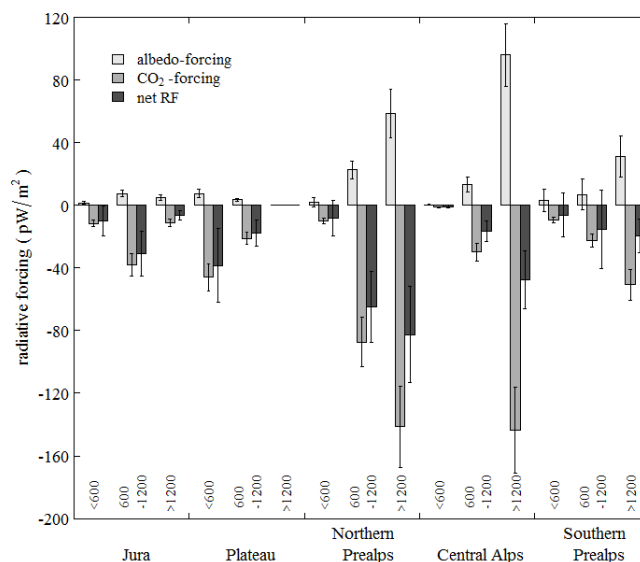
Figure 5. Radiative forcings of the forest expansion between 1985 and 1997 for three elevations in the biogeographical regions Jura, Plateau, northern Prealps, Central Alps and southern Prealps.
