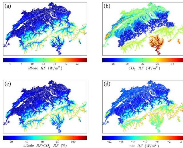
Figure 4. (a) Albedo RF, (b) CO_2 RF, (c) offset: albedo RF/ CO_2 RF and (d) net RF: albedo RF plus CO_2 RF. All data sets were derived for transitions from intensively used open land (< 1000 m) and extensively used open land (> 1000) to closed forest.
