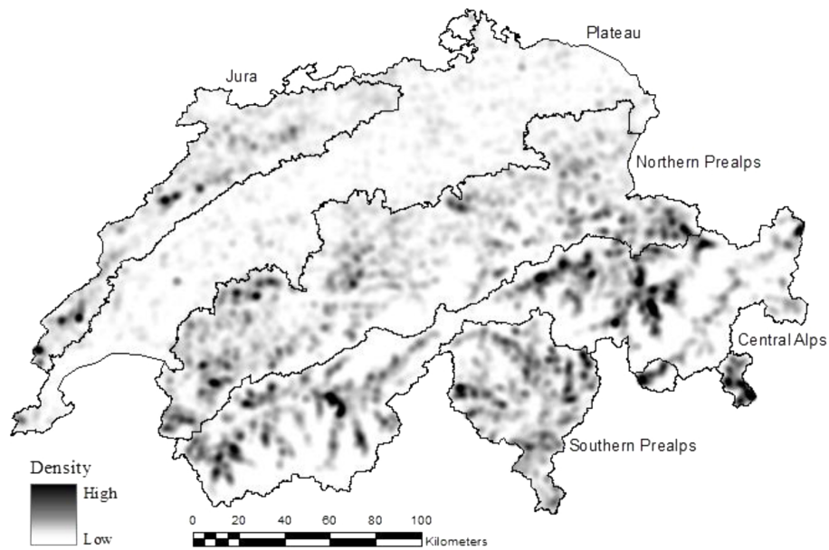
Figure A1. Spatial pattern of forest expansion. The pattern illustrates the density of forest expansion in Switzerland. The density was calculated including the area of all five transitions we used for calculating RF (see Sect. 2.3) and a kernel-density function in ArcGis 10.1 (ESRI).
