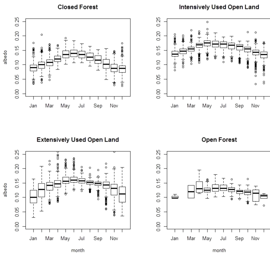
Figure A2. Seasonal variation of albedo values of the four snow-free LULC classes: closed forest, intensively used open land, extensively used open land and open forest (only full BRDF inversion albedo values).
