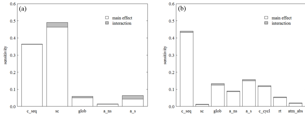
Figure 6. Global sensitivity analysis FAST: (a) sensitivity analysis of spatial variability of c_{seq} (carbon sequestration), s_c (snow cover), glob (global radiation), a_{ns} (albedo difference no snow cover) and a_s (albedo difference snow covered), (b) sensitivity analysis of uncertainty for each pixel: c_{seq} , s_c , glob , a_{ns} , a_s , c_{cycle} (carbon cycle), r_t (radiative transfer) and atm_{absorb} (atmospheric absorption).
