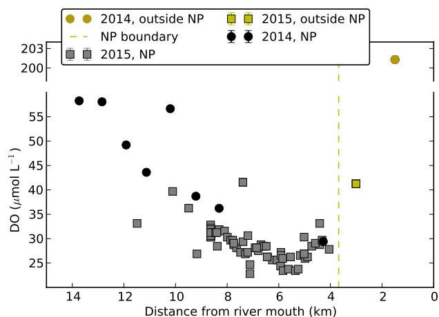
Figure 3. Dissolved oxygen concentrations in the Maludam River. Flow direction is from left to right. Note the discontinuous vertical axis. The yellow markers to the right of the dashed line refer to sampling stations outside the national park.
