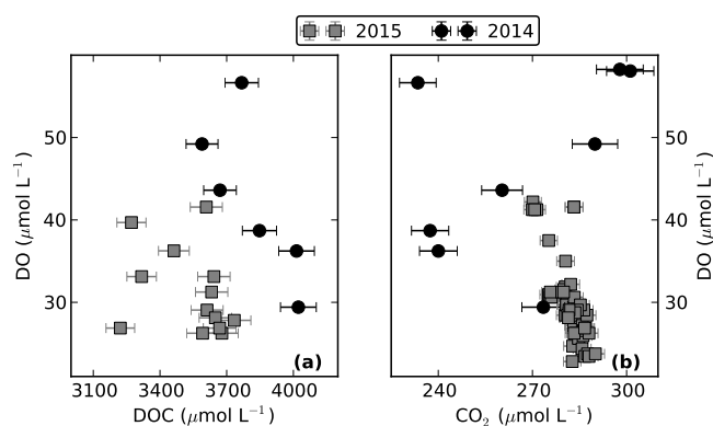
Figure 5. DO vs. DOC (a) and DO vs. \text{CO}_2 (b) reveal a weak linkage between these parameters in the river. The legend applies to both panels.
