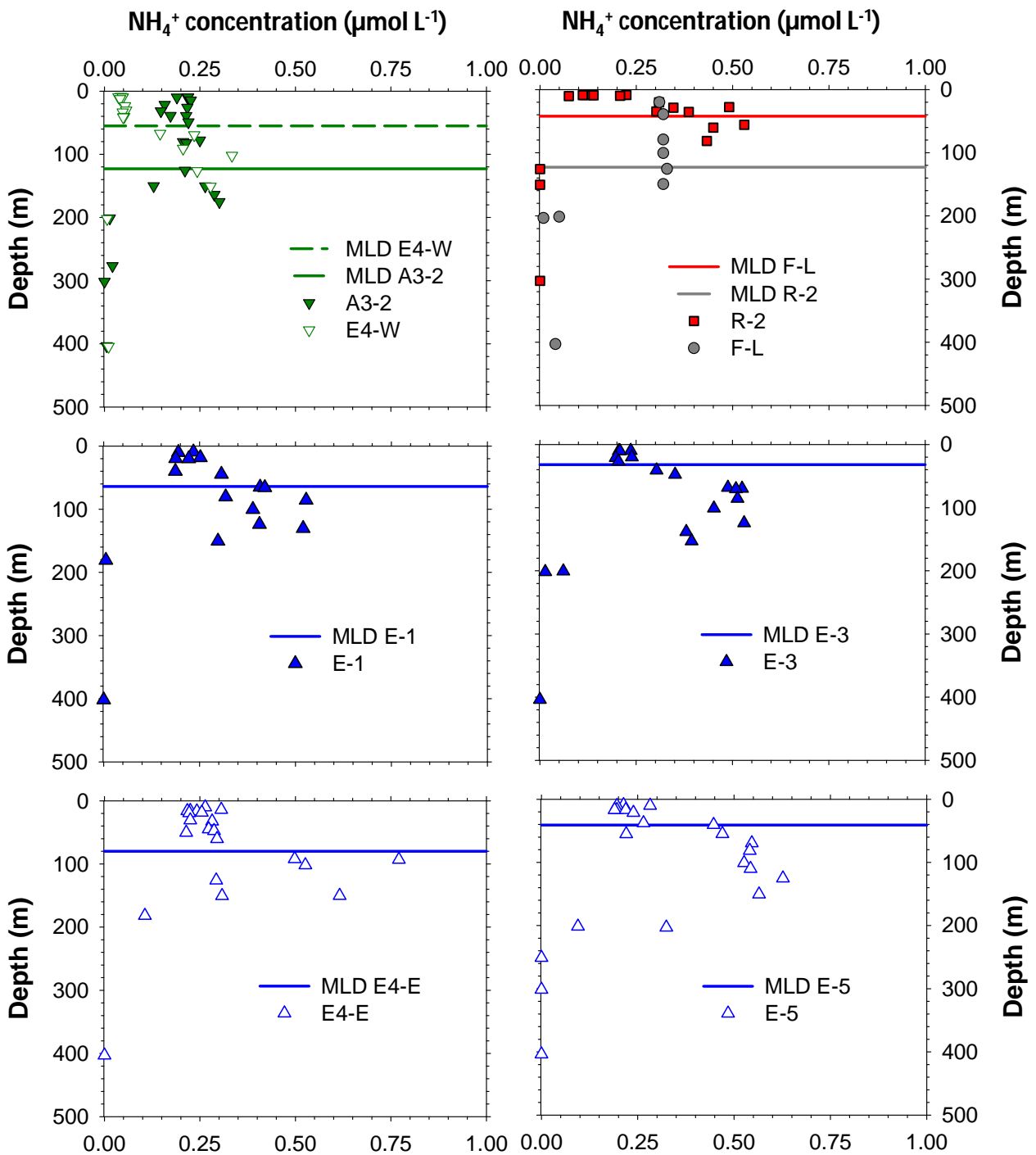
ANNEX: Ammonium concentration ( \mu\text{mol L}^{-1} ) vertical profiles and mixed layer depth (MLD) for (a) A3-2 and E4W, (b) R and F-L, (c) E1, (d) E3, (e) E4E, and (f) E5.
