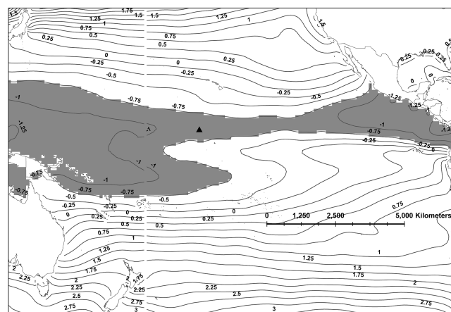
Figure 2. Adjusted oxygen isoscape (shaded in gray). PANWR is depicted by the black triangle. Solid lines are contours of predicted oxygen isotope ratios in barnacle calcite ( \delta^{18}\text{O}_\text{C} ).
