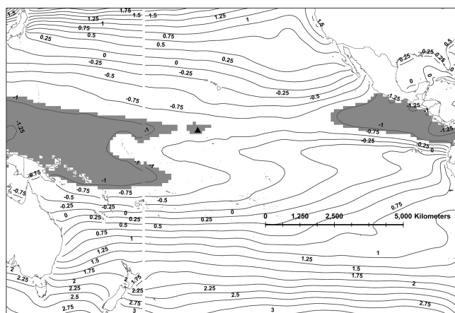
Figure 1. Oxygen isoscape (shaded in gray) showing the area in which we would expect our sea turtles to have resided throughout the life of the barnacles tested. This isoscape was calculated using an oxygen isotope ratio of -0.951 \delta^{18}\text{O}_\text{C} . PANWR is located within this area and depicted by the black triangle. Solid lines are contours of predicted oxygen isotope ratios in barnacle calcite ( \delta^{18}\text{O}_\text{C} ).
