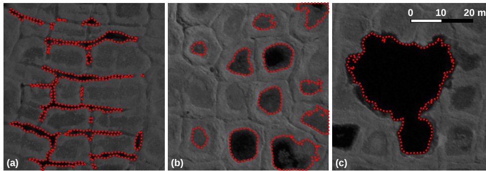
Figure 2. Typical ponds in the polygonal tundra mapped from near infrared (NIR) areal images. At the study site occur (a) ice-wedge ponds, (b) intra-polygonal ponds within intact polygonal structures, and (c) merged ponds show clear signs of degradation of the polygonal structures. According to their degree of degradation intra-polygonal ponds and ice-wedge ponds are classified as initial state ponds (ISPs) and merged ponds as advanced state ponds (ASPs).
