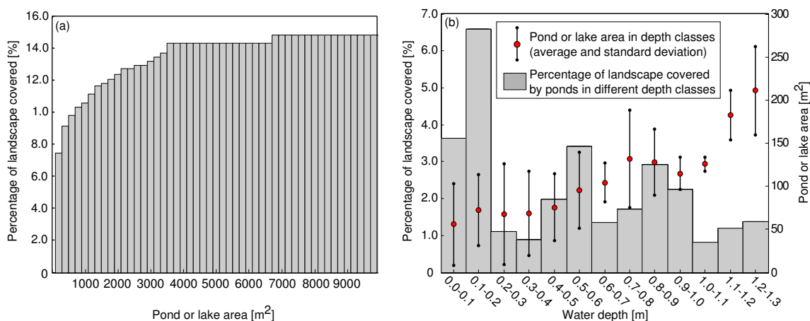
Figure 3. Cumulative percentage of landscape covered by ponds in different size classes (a). Percentage of landscape covered by ponds in different depth classes (b). The secondary y axis in (b) shows the average surface area for each depth class. The whiskers indicate the standard deviation for each depth class.
