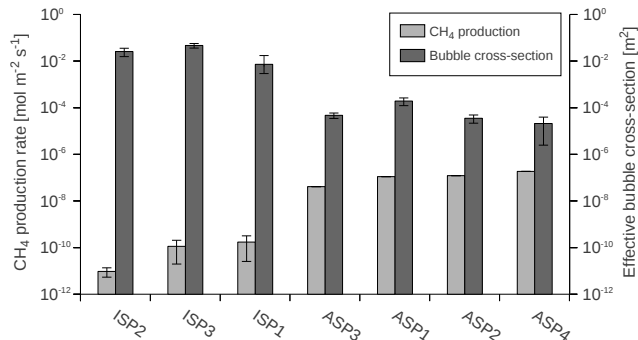
Figure 7. Net methane production and effective bubble cross-section for different ponds, calculated by inverse modeling using the 1-D mass balance model (note the logarithmic scale). The whiskers indicate the 95 % confidence interval of the model results.
