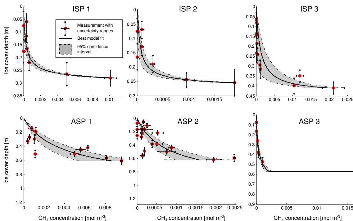
Figure 6. Measured and modeled \text{CH}_4 concentrations with ice cover depth of different ponds. The whiskers show the measurement uncertainty and the shaded areas indicate the 95 % confidence interval of the model. The range of depth axis represents the maximum pond depth. Sampling was limited to a maximum ice cover depth of about 60 cm due to the length of the guide bar used with the chainsaw.
