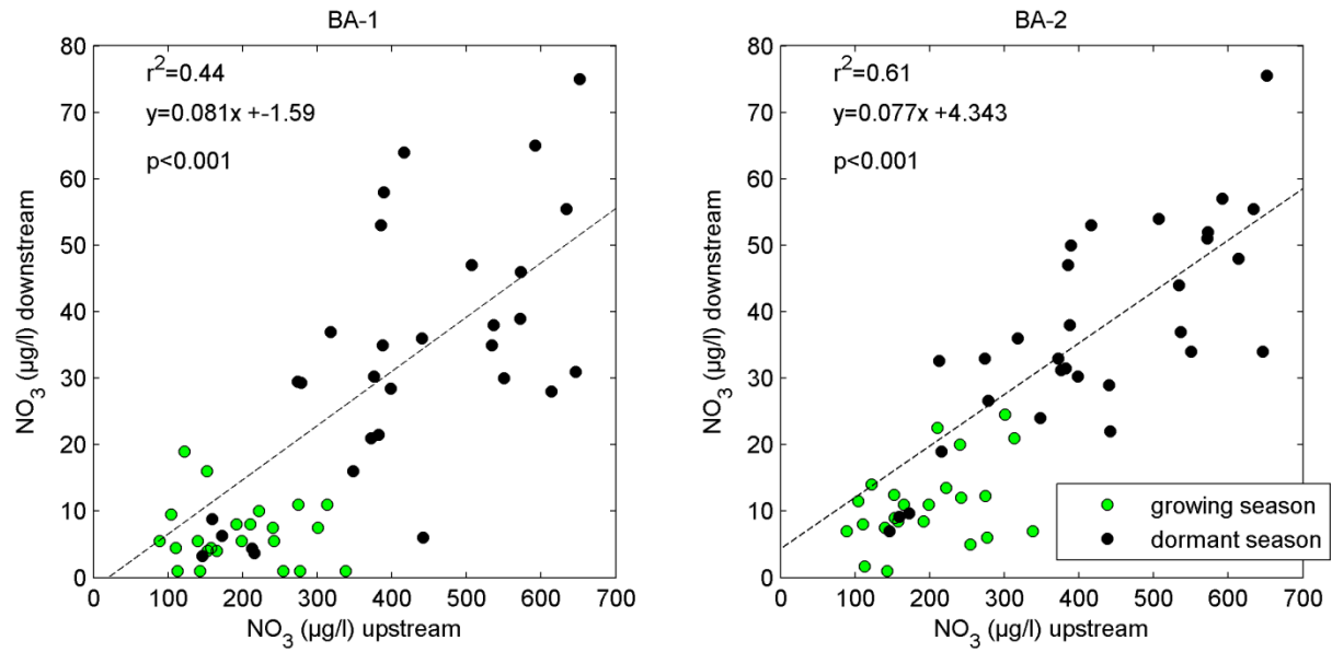
Figure S1: Nitrate ( \text{NO}_3^- ) concentrations at the downstream sites BA-1 (size = 22.9 km 2 ) and BA-2 (size = 8.7 km 2 ) as a function of the concentrations measured at CC-4 clear-cut catchment during 2008-2011. Significant linear relationships were found for the entire dataset (not shown) and the dormant season (shown in figure), whereas no such relationships were found for the growing season.
