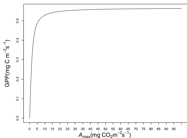
Figure 8. Variation of gross primary production (GPP) with the variation of photosynthetic capacity ( A_{\max} ) from 0 to 100 \text{ mg CO}_2 \text{ m}^{-2} \text{ s}^{-1} . The values of quantum yield ( \alpha ), degree of curvature ( \theta ), ecosystem respiration at reference temperature ( r_0 ), and temperature sensitive parameter ( k_T ) are fixed at 0.7, 0.0022, 0.1, 0.07 respectively. Air temperature ( T_a ) and photosynthetic photon flux density (PPFD) are fixed at 10^\circ\text{C} and 900 \mu\text{mol quanta m}^{-2} \text{ s}^{-1} .
