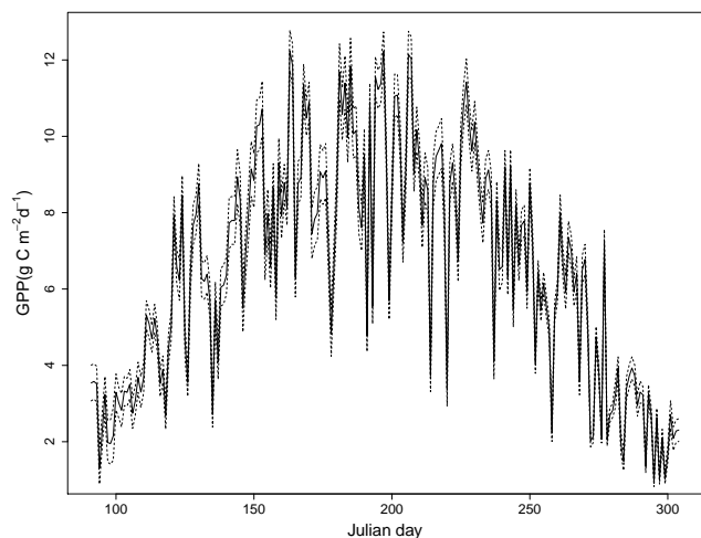
Figure 4. Median (solid line) and 95 % credible intervals (dashed lines) of daily GPP distributions during the growing season of 2009 (1 April to 31 October 2009, Julian days 91 to 304) for the choice of informative prior distributions.
