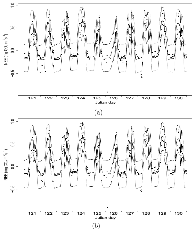
Figure 2. Median (solid lines) and 95 % credible intervals (dashed lines) of the posterior distribution of NEE together with half-hourly NEE measurements (solid points) for a 10-day block (1 May to 10 May 2009, Julian days 121 to 130): (a) when using informative prior distributions, (b) when using non-informative prior distributions.
