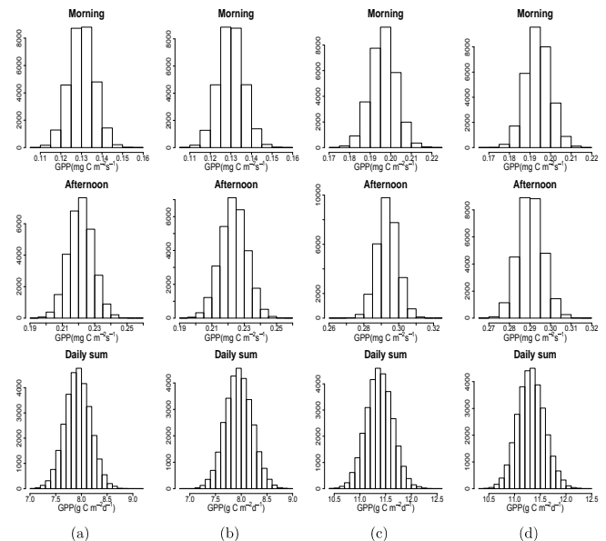
Figure 3. Histograms of half hourly GPP (Morning and afternoon) and daily sum of GPP when using the following: (a) informative priors on Julian day 121 (1 May 2009), (b) non-informative priors on Julian day 121, (c) informative priors on Julian day 196 (15 July 2009), (d) non-informative priors on Julian day 196. The morning and afternoon time belong to half-hour 08:00 to 08:30 and 13:00 to 13:30 CET respectively. The y axis is frequency; CET is Central European Time.
