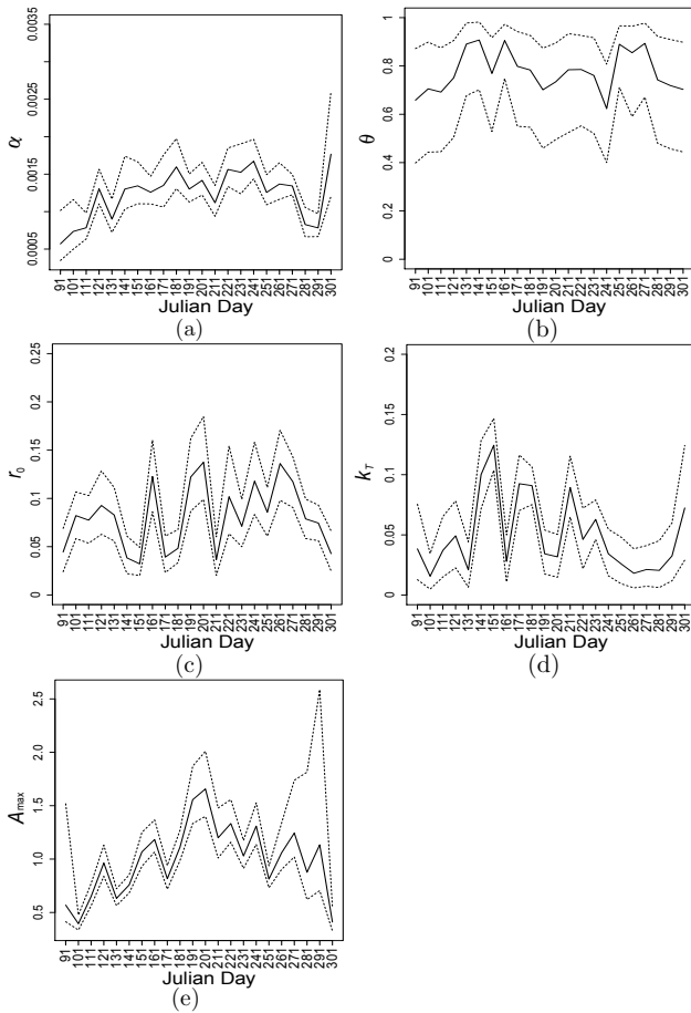
Figure 6. Median (solid lines) and 95 % credible intervals (dashed lines) of the posterior distributions of the NRH parameters when using informative prior distributions for each 10-day block during the growing season in 2009. The x axis is the first Julian day of each 10-day block. The y axis represents NRH parameter. Information about the NRH parameters is given in Table 1.
