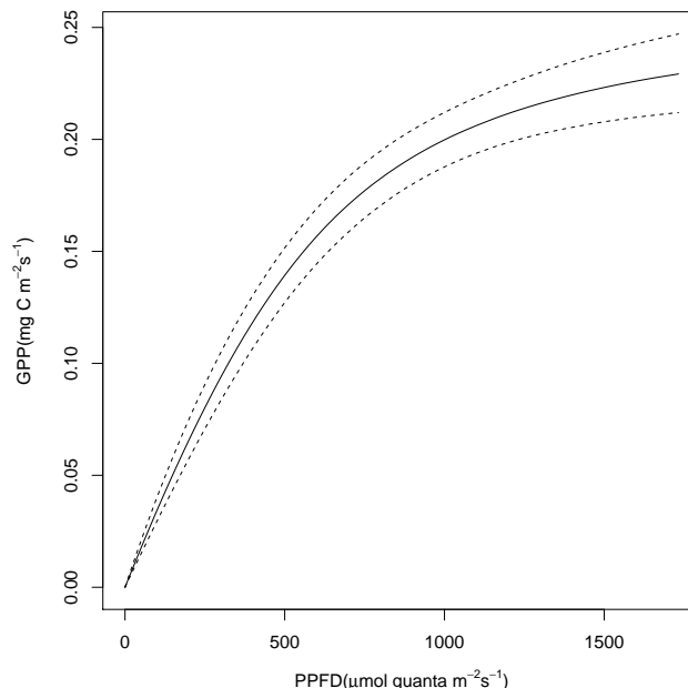
Figure 5. Median (solid line) and 95 % credible intervals (dashed lines) of half-hourly gross primary production (GPP) with photosynthetic photon flux density (PPFD) for a 10-day block (1 May to 10 May 2009, Julian days 121 to 130) for the choice of informative prior distributions.
