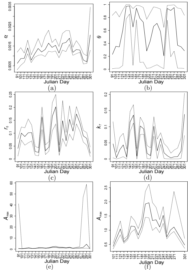
Figure 7. As Fig. 6 when using non-informative prior distributions. To help the visualization of A_{\max} we have added a subfigure (f) with the spikes removed (i.e., without the blocks of Julian days 91–100, 281–290, and 291–300).
