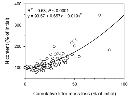
Figure 5. Second-order polynomial relationship between the cumulative litter mass loss (in percentage of initial) of leaf litter of Pinus sylvestris (Hyytiälä, Finland), Pinus sylvestris (Männikjärve, Estonia), Fagus sylvatica (Sorø, Denmark), and Pseudotsuga menziesii (Speulderbos, Netherlands), Lolium perenne (Easter Bush, UK) and Festuca pseudovina (Bugac, Hungary) and the litter N content relative to initial during a reciprocal litter translocation decomposition experiment. Data points ( n = 136 ) are the average value of three replicate litter bags.
