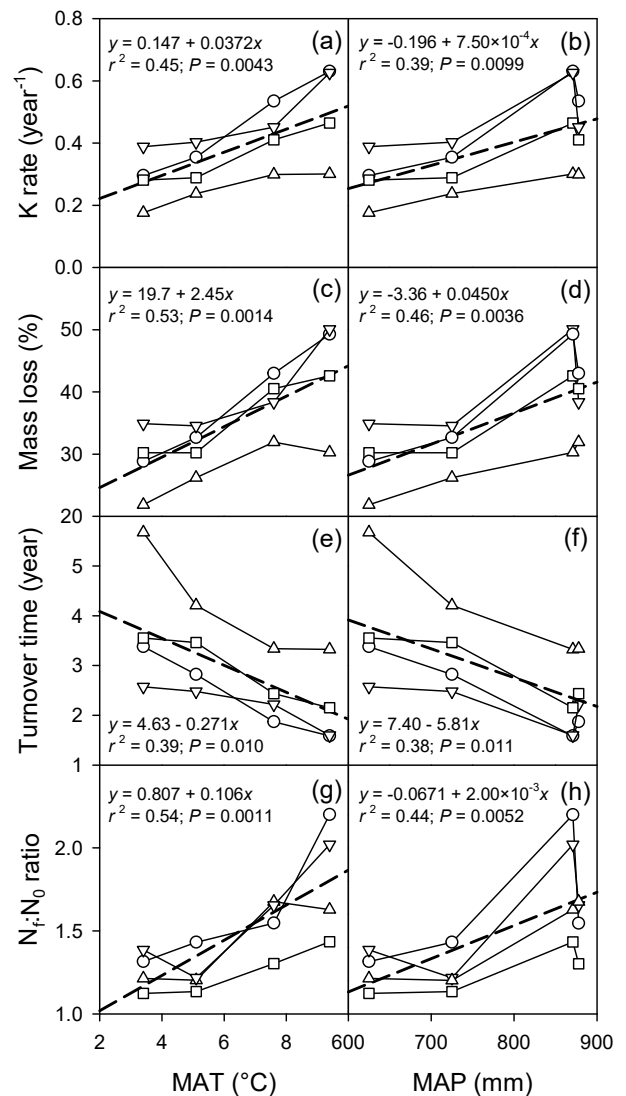
Figure 3. Litter decomposition traits of four different tree litter species with different origin decomposed in four European sites with different mean annual temperature ( T_a ) and mean annual precipitation ( P ). Symbols as in Fig. 1. Data corresponding to the same origin of litter are connected with a solid line to visually evaluate the evolution of the trait across the T_a and P range. The dashed line represents the Pearson's linear regression best fit of all the data. Traits are first-year decomposition k rate (a, b), percentage of mass loss after 1 year of decomposition relative to initial mass (c, d), estimated litter turnover time (e, f), and ratio between final litter N content ( N_f ) after 1 year of decomposition and the initial nitrogen content ( N_0 ).
