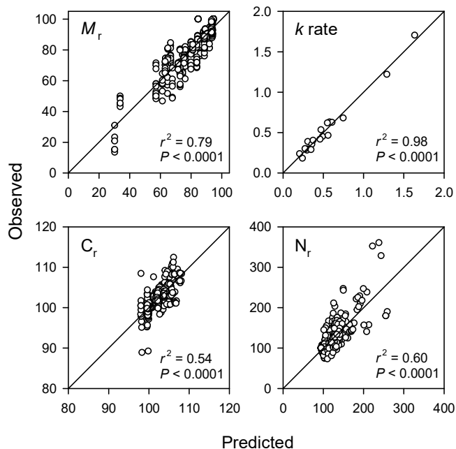
Figure 6. Modelled data using Eqs. (2–8) plotted against observed data: ( M_r ) the percentage of remaining litter mass relative to the initial value, ( k rate) litter decomposition rate constant, and the percentage of carbon ( C_r ) and nitrogen ( N_r ) content in litter relative to the initial value. For reference see 1 : 1 solid lines.
