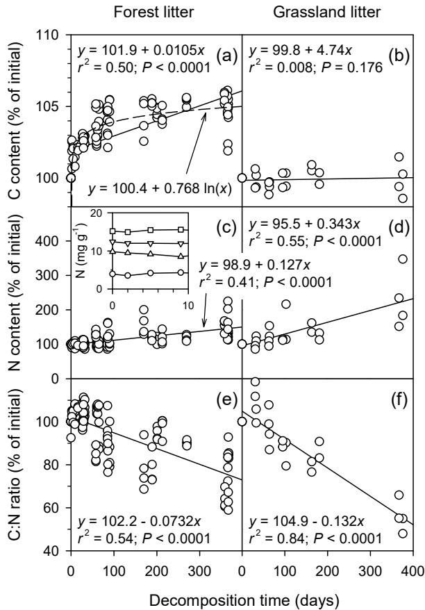
Figure 4. Total C, N and C:N ratio relative to the initial level at the beginning of the decomposition period. The data correspond to reciprocal litter translocation experiments with leaf litter from forests sites: Pinus sylvestris (Hyytiälä, Finland), Pinus sylvestris (Männikjärve, Estonia), Fagus sylvatica (Sorø, Denmark), and Pseudotsuga menziesii (Speulderbos, Netherlands); and grassland sites: Lolium perenne (Easter Bush, UK) and Festuca pseudovina (Bugac, Hungary). Data points ( N = 112 for tree litter and N = 24 for grass litter) are the average value of three litter bags. In (a), the dashed line represents the best logarithmic fit to the data. The inset in (c) represents the N content in leaf litter during the first 10 days of decomposition. Symbols stand for P. sylvestris from Hyytiälä (○) and Männikjärve (▽), F. sylvatica (Δ), and P. menziesii (□).
