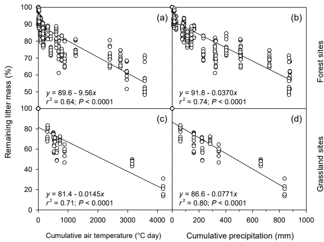
Figure 2. Average remaining biomass during first year decomposition of leaf litter of four tree species in four forest sites (a, b) and grass litter from two species in two grasslands (c, d) across Europe (see Table 1 for details). The cumulative air temperature is the sum of daily average temperatures above 0 °C from the beginning of the decomposition period until the date of litter collection for every litter bag. The cumulative precipitation is the sum of daily precipitation (in mm) from the beginning the decomposition period until the date of litter collection. The solid lines represent the Pearson's linear regression best fit ( n = 336 for forest sites and n = 72 for grassland sites).
