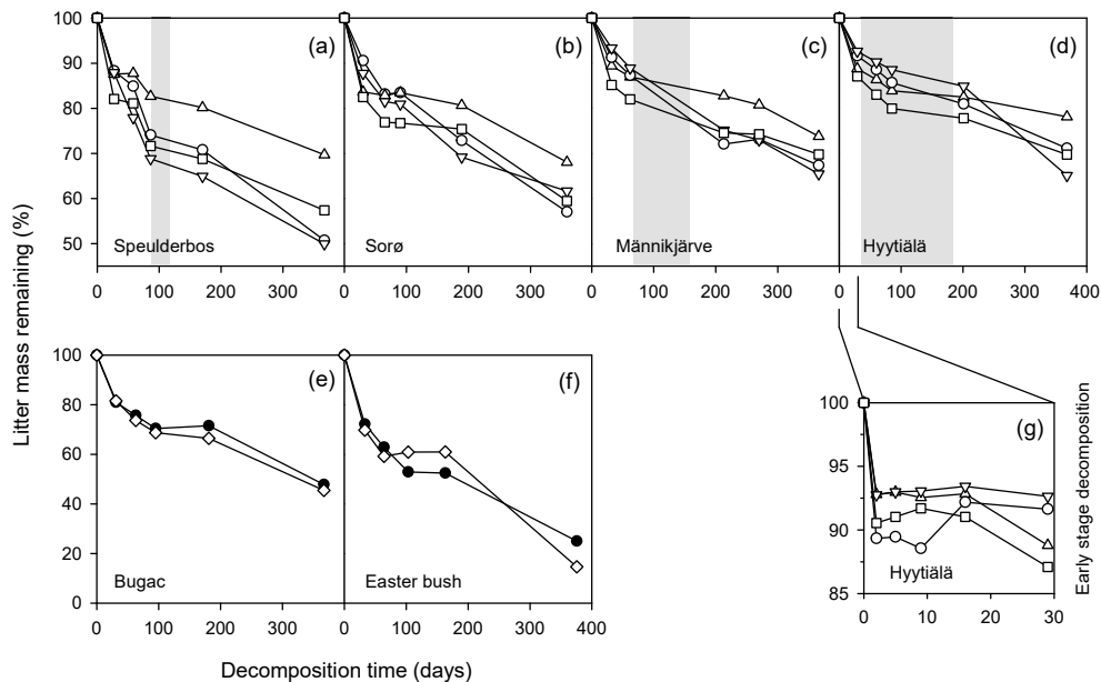
Figure 1. Average remaining leaf litter mass during a reciprocal litter transplantation experiment of four tree litter types during decomposition in four forest sites ( a, b, c, d ) and grass litter types during decomposition in two grassland sites ( e, f ). Different symbols stand for different sites of litter origin (and typically a different species, except the northernmost sites Hyttiälä and Männikjärve): Pinus sylvestris (○) from Hyttiälä (Finland), P. sylvestris (▽) from Männikjärve (Estonia), Fagus sylvatica (Δ) from Sorø (Denmark), Pseudotsuga menziesii (□) from Speulderbos (Netherlands) ( e ) Festuca pseudovina (◇) from Bugac (Hungary) and ( f ) Lolium perenne (●) from Easter Bush (UK). Data points are the average of three replicate litter decomposition bags (maximum standard error between replicates during the decomposition of 4.7 %, not plotted). The shadowed areas correspond to the winter period where the litter bags were covered by a snow layer of at least 3 cm. ( g ) corresponds to early-stage decomposition for tree litter types in Hyttiälä. Table 1 provides details of the sample sites and litter characteristics.
