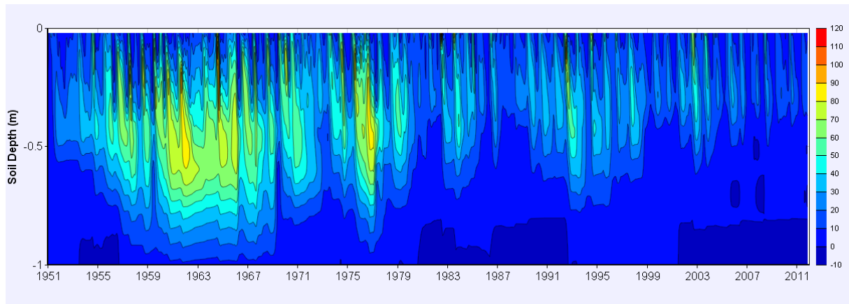
Supplementary Figure 1. The simulated soil nitrate concentration ( \text{mg N l}^{-1} ) distribution across the soil profile (down to 1 m depth).
