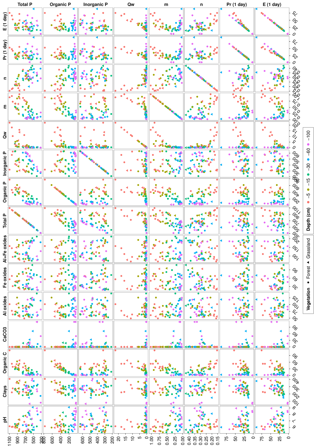
Figure S3: Matrix of scatter plots of P parameters plotted against soil physico-chemical properties, other P parameters and fine root densities. Q_w : phosphate ions in solution; m and n are the fitting parameters of Eq. 4; Pr : diffusible phosphate ions; E : isotopically exchangeable phosphate ions; FRLD: fine root length density; FRMD: fine root mass density.
