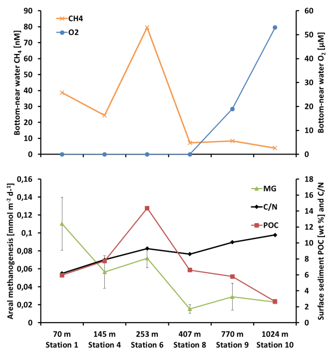
Figure 6. Bottom-near water methane ( \text{CH}_4 ) and oxygen ( \text{O}_2 ) concentrations along the depth transect (above). Surface sediment particulate organic carbon (POC) content and C / N ratio together with integrated methanogenesis (MG) rates (0–25 cm b.s.f.) along the depth transect (below). For MG rates, averages are shown with standard deviation beside St. 10, where a mean from two replicates is shown (see text). Please note the secondary y axis.
