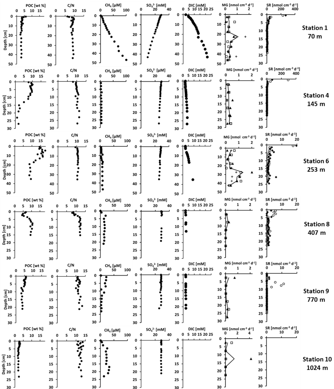
Figure 2. Profiles of particulate organic carbon (POC), C/N ratio, methane ( \text{CH}_4 ), sulfate ( \text{SO}_4^{2-} ), DIC (dissolved inorganic carbon), net methanogenesis (MG) rates and sulfate reduction (SR) rates in the MUC cores along the depth transect. For MG, triplicates (symbols) and mean (solid line) are shown. For SR, duplicates are shown. Data points from the overlaying water in the MUC core (OLW) are set to 0 cm. Note deviant scale dimension for MG at St. 6 and for SR at St. 1 and 2.
