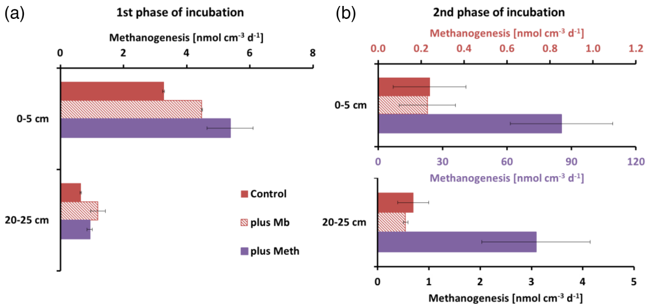
Figure 4. Potential methanogenesis rates in sediment slurry experiments from the two sediment intervals (0–5 and 20–25 cm) at St. 1 (70 m). The first phase of the incubation shows rates calculated from day 0–5 (a), while the second phase of the incubation summarizes the rates from day 8–23 (b). “Control” is the treatment with sulfate-rich (28 mM) artificial seawater medium, “plus Mb” is the treatment with sulfate-rich artificial seawater medium plus molybdate (Mb, 22 mM), and “plus Meth” is defined as the treatment with sulfate-rich artificial seawater medium plus methanol (Meth, 10 mM). Per treatment, average values are shown with standard deviation. Please note the split-up in the diagram in (b) and the different x axis for methanogenesis.
