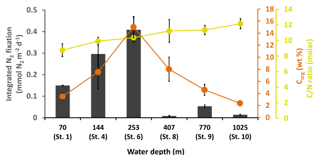
Figure 5. Integrated nitrogen fixation (mmol N 2 m -2 d -1 , grey bars, average of three replicates), average organic carbon content (C org , wt %, orange curve) and the average C/N molar ratio (yellow curve) from 0 to 20 cm along the depth transect (m). Error bars indicate standard deviation.
