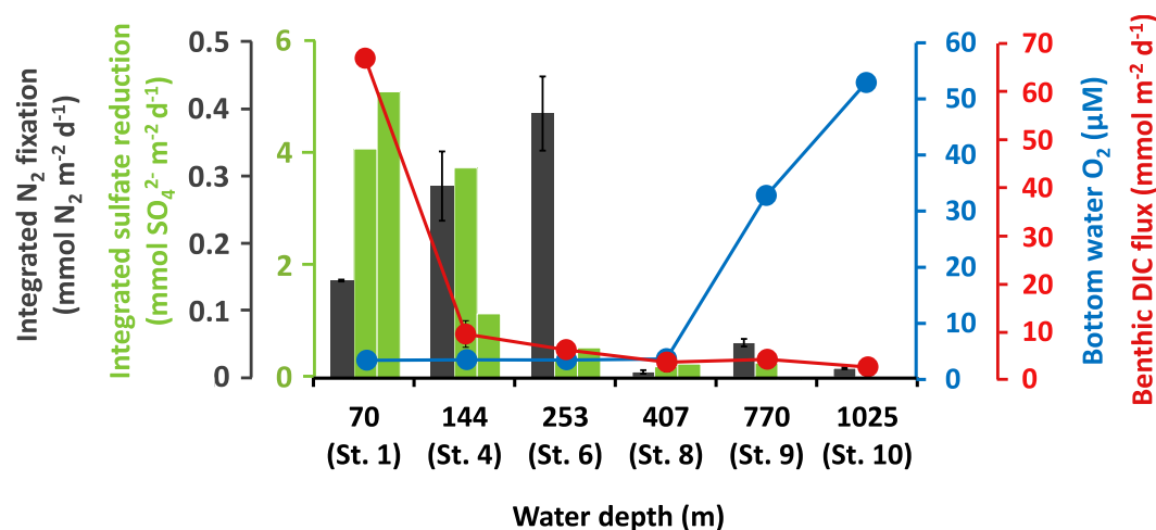
Figure 4. Integrated nitrogen fixation (mmol N 2 m -2 d -1 , grey bars, average of three replicates) and integrated sulfate reduction (mmol SO 4 2- m -2 d -1 , green bars, two replicates) from 0 to 20 cm, including dissolved inorganic carbon flux (DIC, mmol m -2 d -1 , red curve from Dale et al., 2015) and bottom water O 2 (μM, blue curve) along the depth transect (m). Error bars indicate standard deviation of N 2 fixation.
