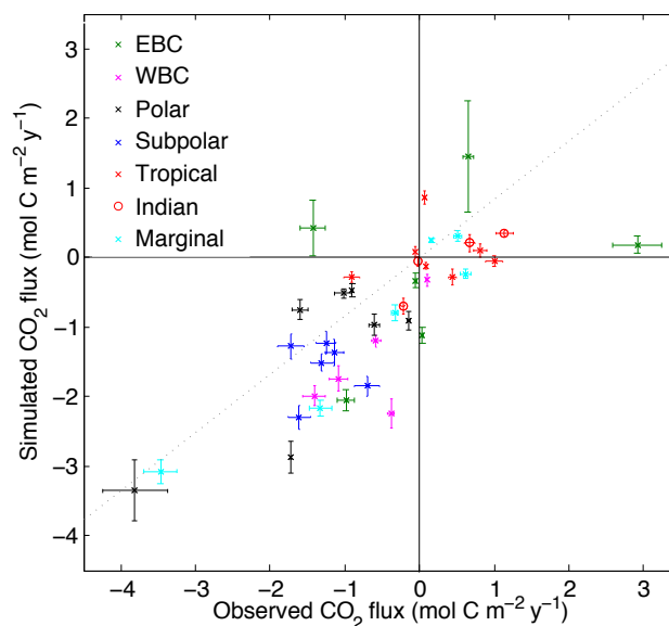
Figure 6. Simulated vs. observed MARCATS sea-to-air flux of total carbon in \text{mol C m}^{-2} \text{yr}^{-1} . Vertical error bars show the standard deviation from the 1993–2012 interannual variability for model results and the horizontal bars correspond to the 1990–2011 variability from computational methods used in LA14 for observation-based estimates. Here, regression line (grey dotted) has y intercept forced to 0. All MARCATS regions have been used except the Black Sea, the Persian Gulf (no data estimate), and the Sea of Okhotsk (see text).
