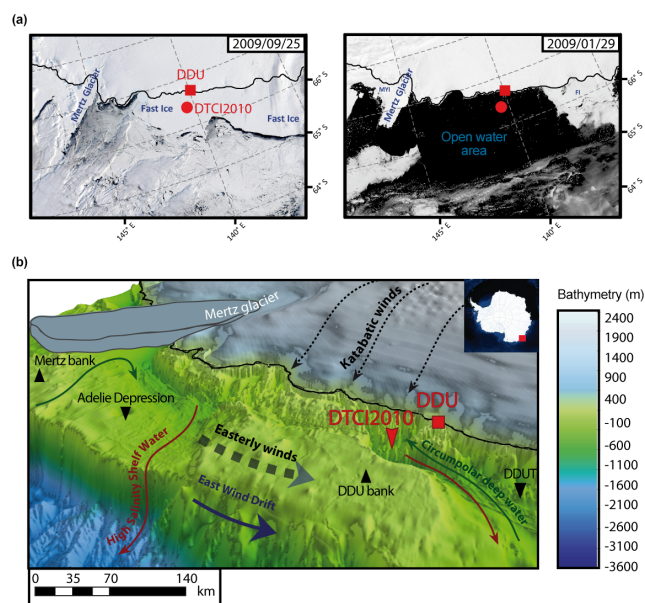
Figure 1. Study area. (a) Modis satellite images of Adélie Land, showing mean sea ice conditions from early spring to summer in the region, the location of sediment core DTCI2010 and the French research station Dumont D'Urville (DDU). (b) Map of the study area showing the location of sediment core DTCI2010 in the Dumont D'Urville Trough (DDUT), the main glacial and topographic features, the principal water masses (solid lines) and the main wind streams (dashed lines).
