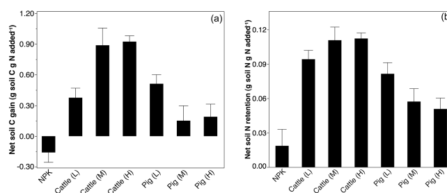
Figure 4. Relationships between (a) net soil C gain (i.e. grams of C gained in the soil) and (b) net soil N retention (i.e. grams of N retained in the soil) per gram of N added over 43 years under each nutrient treatment. Abbreviations as in Fig. 1. Standard errors indicate variation among six replicate values for each treatment.
