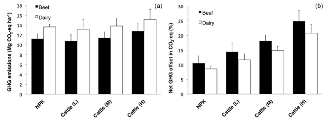
Figure 6. Overall GHG emissions (in \text{CO}_2\text{-eq} ) based on different nutrient treatments (a) and percentage of GHG emissions that can be offset by soil C sequestration associated with long-term inorganic and organic nutrient additions. Estimates refer to dairy and beef farming systems and are calculated as net contribution of multiple GHGs (i.e. global warming potential; see Supplement). Abbreviations as in Fig. 1. Standard errors indicate variation among six replicate values for each treatment.
