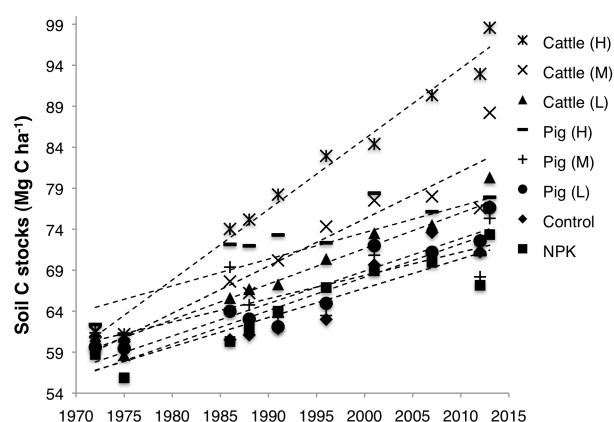
Figure 1. Changes in soil C stocks from 1970 to 2013 (0–15 cm soil depth) under either organic or inorganic nutrient additions or no nutrients (i.e. control). Nutrient application rates: NPK = 200 kg N, 32 kg P, 160 kg K \text{ha}^{-1} \text{ yr}^{-1} ; Pig (L), Pig (M) and Pig (H) = Pig slurry applications at 50 (low), 100 (medium) and 200 (high) \text{m}^3 \text{ ha}^{-1} \text{ yr}^{-1} respectively; Cattle (L), Cattle (M), Cattle (H) = Cattle slurry applications at 50 (low), 100 (medium) and 200 (high) \text{m}^3 \text{ ha}^{-1} \text{ yr}^{-1} respectively. Best fit linear functions (dashed lines): NPK ( y = 0.36x - 647 ; R^2 = 0.87 ); control ( y = 0.41x - 746 ; R^2 = 0.83 ); Pig (L) ( y = 0.39x - 723 ; R^2 = 0.88 ); Pig (M) ( y = 0.28x - 498 ; R^2 = 0.65 ); Pig (H) ( y = 0.31x - 546 ; R^2 = 0.67 ); Cattle (L) ( y = 0.43x - 796 ; R^2 = 0.91 ); Cattle (M) ( y = 0.65x - 1230 ; R^2 = 0.95 ); Cattle (H) ( y = 0.86x - 1636 ; R^2 = 0.98 ).
