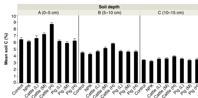
Figure 3. Relationship between mean soil C (%) content at three soil depths (A = 0–5 cm, B = 5–10 cm, C = 10–15 cm) and different nutrient treatments as averaged for two recent years (2012 and 2013). Abbreviations as in Fig. 1. Standard errors indicate variation among six replicate values for each treatment.
