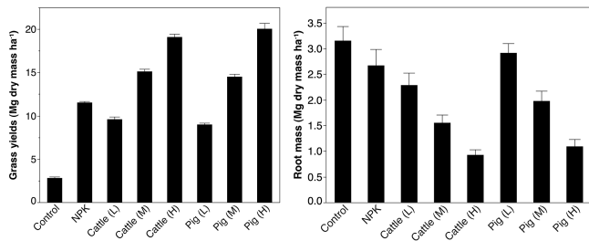
Figure 5. Relationships between (a) grass yields (averaged for five recent years 2009–2013) and (b) total root mass (measured in 2014 between 0 and 20 cm soil depth) and the different nutrient treatments. Abbreviations as in Fig. 1. Standard errors indicate variation among six replicate values for each treatment.
