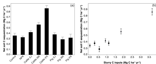
Figure 2. Relationship between net soil C sequestration rates (Mg C ha -1 yr -1 ; 0–15 cm depth) and (a) nutrient application treatments, (b) C inputs from animal slurry (Mg C ha -1 yr -1 ). Experimental treatments same as in Fig. 1. Symbols: square = no C inputs (control plots), circles = C inputs from pig slurry, triangles = C inputs from cattle slurry. Standard errors indicate variation among six replicate values for each treatment.
