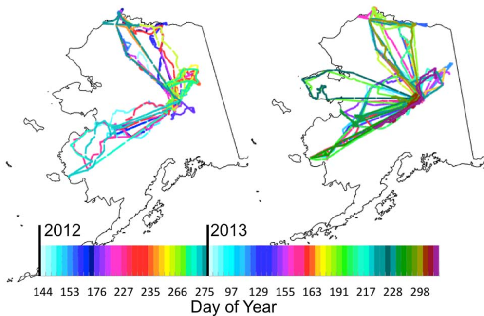
Fig. S1. Flight tracks with valid CH 4 mole fractions during the CARVE 2012 and 2013 campaigns. There were 31 flight days in 2012 and 43 flight days in 2013 (Supplement Table S2).
