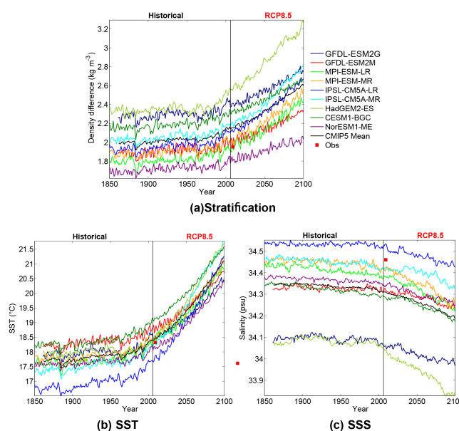
Figure 1. Time series of global mean surface stratification, SST and SSS for historical and RCP8.5 over 1850–2100. Surface stratification is defined as the density difference between 200 m and the surface. Red square indicates observations from the WOA2009 data.
