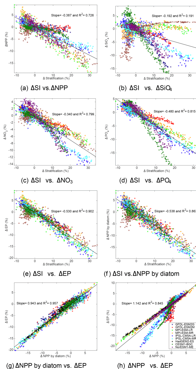
Figure 7. Relationships are shown between the relative percent change in surface stratification with climate and the relative change in several biogeochemical variables including net primary production (NPP) (a), silicate (b), nitrate (c), phosphate (d), export production (EP) (e), the fraction of NPP by diatoms (f). EP is plotted against the change in the fraction of NPP by diatoms (g) and against the change in NPP (h). All changes are relative to the 1990s and plotted over 1850–2100. These time series are derived from global annual mean data.
