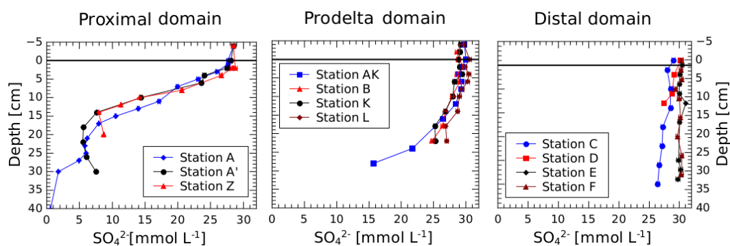
Figure 8. Sulfate profiles measured in the porewaters (mmol L -1 ) of the proximal, the prodelta and in the distal domains.
