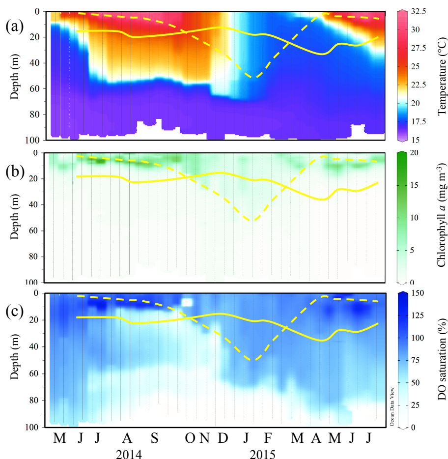
Figure 2. Seasonal variability in (a) temperature (°C), (b) chlorophyll a concentration ( \text{mg m}^{-3} ), and (c) dissolved oxygen saturation (%) from S1 in the Feitsui Reservoir (Fig. 1). Profile data were normally collected on weekly basis throughout the warmer months and every 2 weeks in winter. Solid yellow line indicates the limit of euphotic zone and dashed yellow line the depth of mixed layer.
