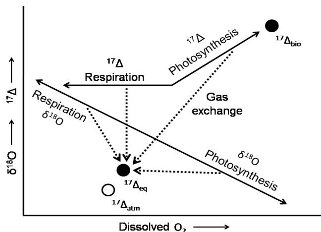
Figure 5. A schematic diagram showing the effects of photosynthesis, respiration, and air–water gas exchange on dissolved O 2 concentrations, \delta^{18}\text{O} and ^{17}\Delta . \delta^{18}\text{O} changes with all the processes and additionally is also affected by mixing. Because of non-mass-dependent processes occurring in the stratosphere, the ^{17}\Delta of O 2 in air has a different signal to the O 2 produced biologically where fractionation is mass-dependent. ^{17}\Delta increases due to photosynthesis, decreases due to gas exchange but is not affected by respiration. Respiration removes O 2 and decreases the dissolved O 2 concentration but fractionates O 2 isotopes in a mass-dependent way, which does not affect the relative proportion of \delta^{17}\text{O} and \delta^{18}\text{O} and therefore the ^{17}\Delta . ^{17}\Delta_{\text{bio}} is the maximum value of pure biological signal, which amounts to ^{17}\Delta of water. The slope of ^{17}\Delta increase towards ^{17}\Delta_{\text{bio}} is the kinetic slope \lambda for respiration ( \lambda = 0.518 ). ^{17}\Delta_{\text{eq}} is the O 2 at air–water equilibrium, which has a small offset from ^{17}\Delta_{\text{atm}} , which is by definition 0, due to fractionation at equilibrium where \delta^{17}\text{O} and \delta^{18}\text{O} slopes during invasion and evasion follow a slightly different slope to that of respiration.
