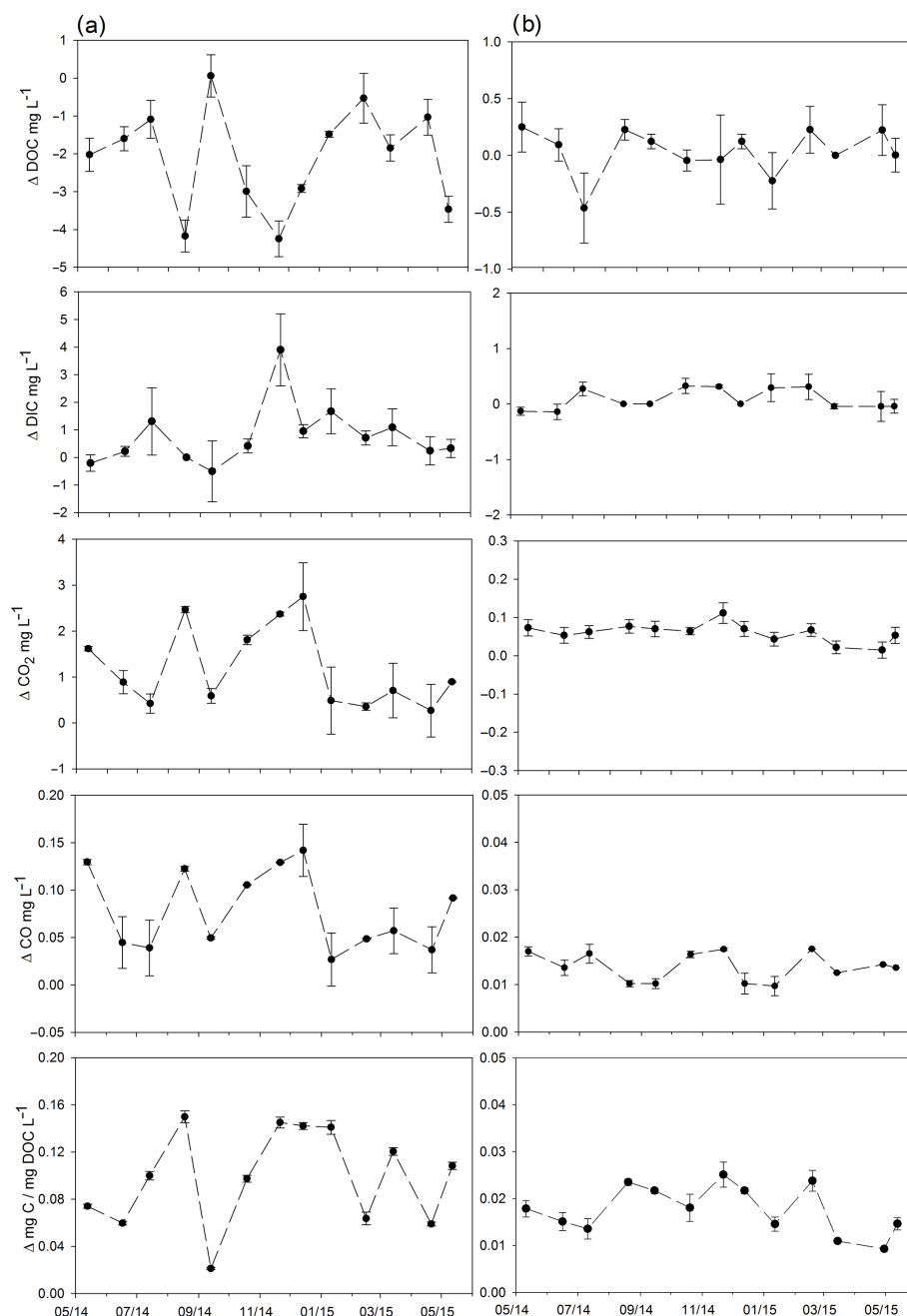
Figure 4. Irradiation-induced changes to carbon species DOC, DIC, CO 2 and CO in monthly water samples from panel Black Burn (a) and Loch Katrine (b). DOC normalised changes to all C species changes (photoreactivity, quantified as explained in the text) are shown on the bottom row. Data represent the difference between the mean of irradiated and unirradiated control samples. Error bars show the standard error of the mean ( n = 4 ). Note different y axis scales for Black Burn and Loch Katrine water samples.
