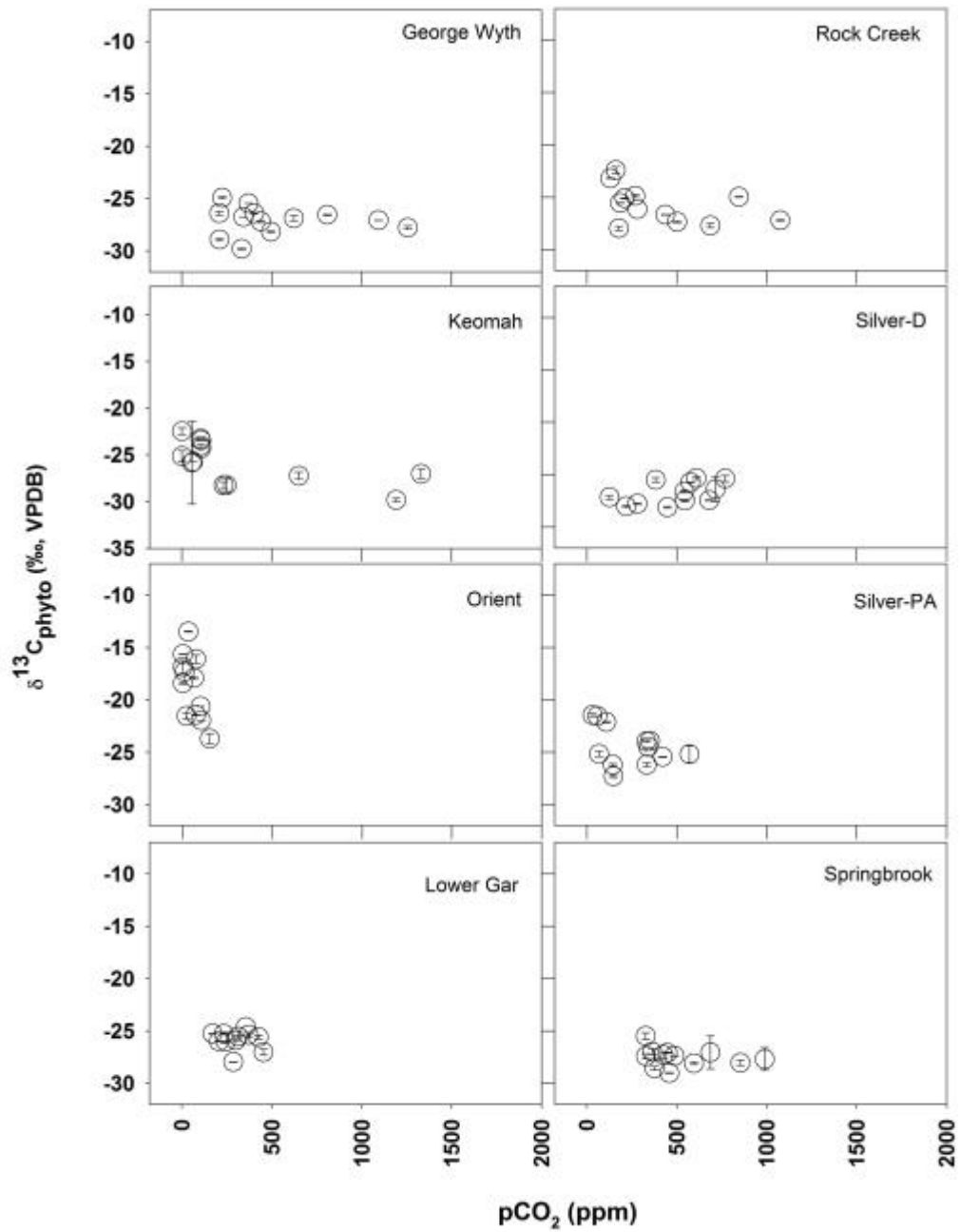
Figure S2. Phytoplankton isotopic composition and ambient \text{pCO}_2 concentration for lakes George Wyth, Keomah, Orient, Lower Gar, Rock Creek, Silver (Dickinson Co.), Silver (Palo Alto Co.), and Springbrook.
