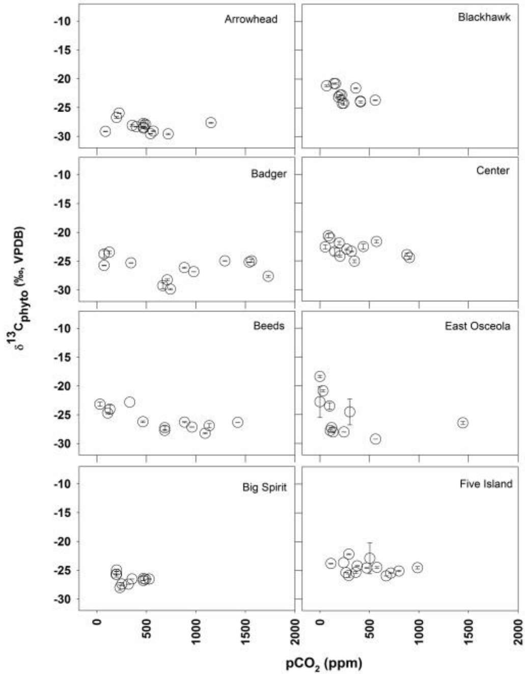
Figure S1. Phytoplankton isotopic composition and ambient \text{pCO}_2 concentration for lakes Arrowhead, Badger, Beeds, Big Spirit, Blackhawk, Center, East Osceola, and Five Island.
