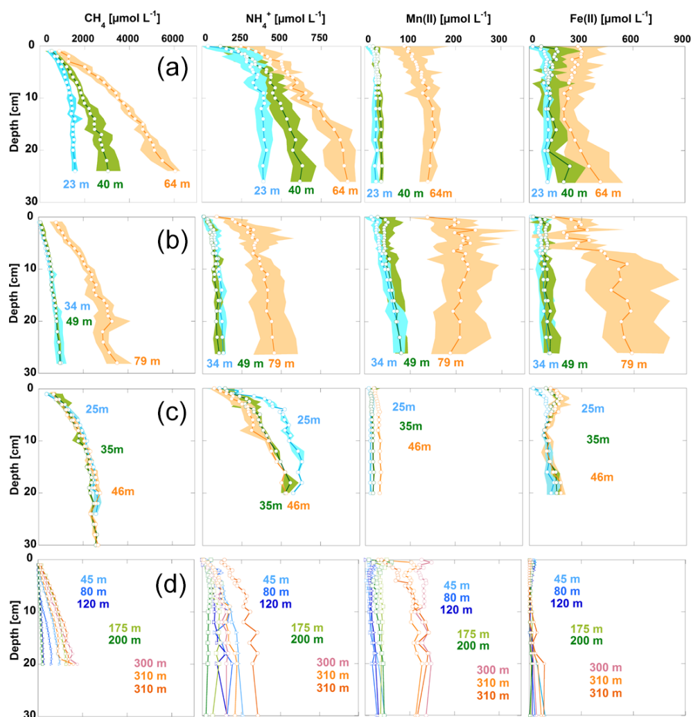
Figure 1. Porewater concentration profiles of \text{NH}_4^+ , \text{CH}_4 , \text{Mn(II)} , and \text{Fe(II)} from (a) Lake Baldegg, (b) Lake Aegeri, (c) Lake Hallwil, and (d) Lake Geneva. Bold lines are averaged values of up to five measurements, while the areas of corresponding colors show the range of minimal and maximal values. Coring sites of Lake Geneva (d) were sampled only once.
