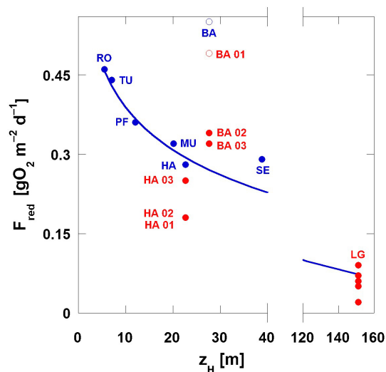
Figure 3. Average fluxes of reduced compounds from the sediments of eight meso- to eutrophic lakes decrease systematically with mean hypolimnion depth ( z_{\text{H}} ), except for sediments sampled at the deepest sites of lakes with pronounced sediment focusing (BA, BA 01, open circles). F_{\text{red}} values of Lake Baldegg (BA01 to 03) show a significant increase with sampling depth due to strong sediment focusing. Blue circles indicate data for Rotsee (RO), Türlensee (TU), Pfäffikersee (PF), Lake Murten (MU), and Lake Sempach (SE), taken from Müller et al. (2012a), while red circles show data of the current study. Meromictic Lake Zug is not shown. The blue line is used to guide the eye.
