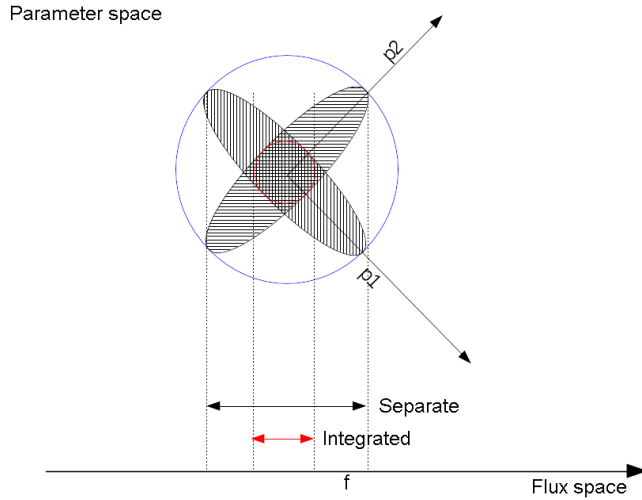
Figure 2. Schematic illustration of PDFs in parameter space (upper section) and flux space (lower section). Prior parameter PDF in blue. Posterior PDFs for separate (integrated) QND in black (red). Projections onto posterior flux uncertainty with QND for either component network (black) or integrated QND (red).
