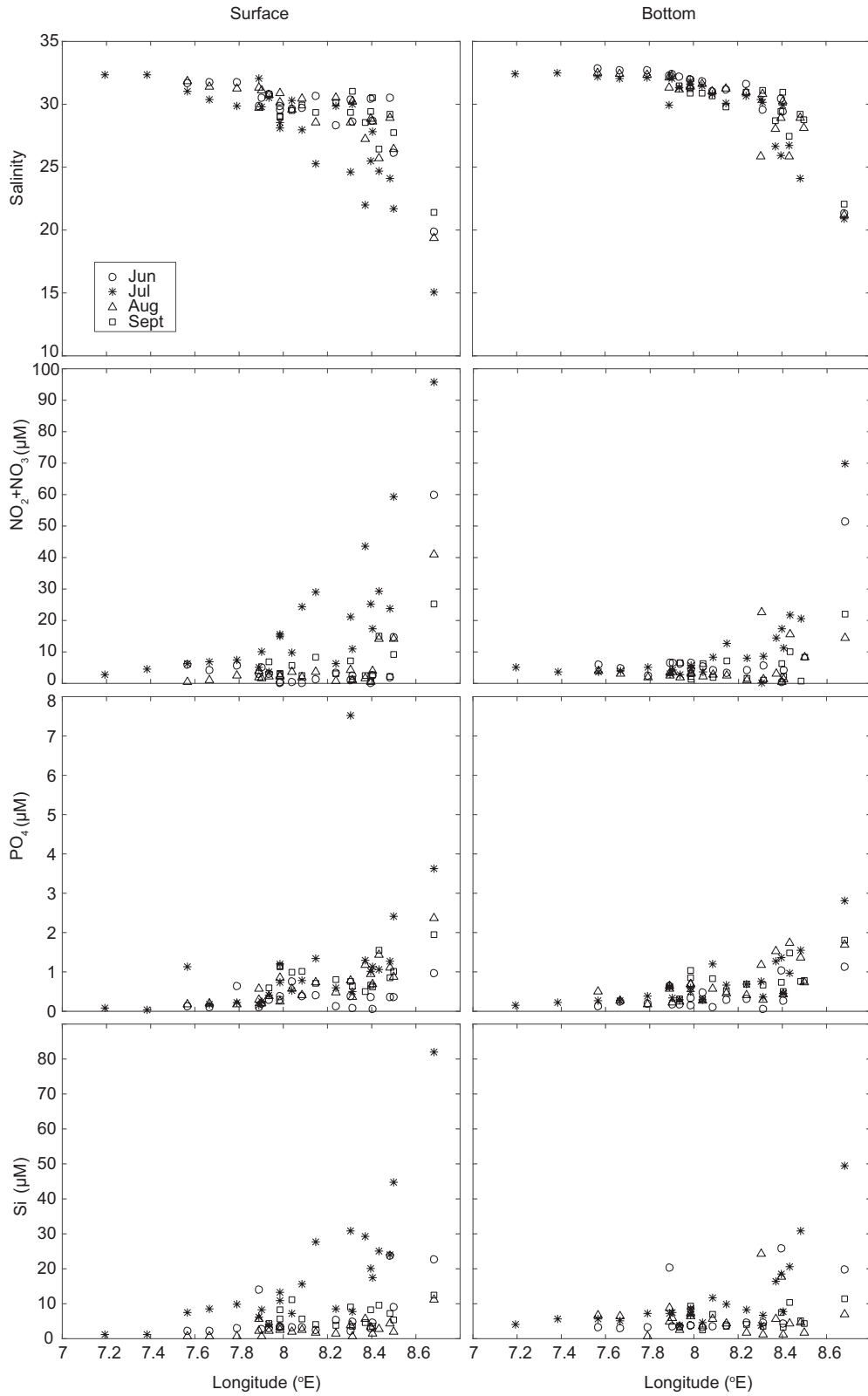
Fig. S2. Surface (left panels) and bottom (right panels) salinity, nitrate + nitrite ( \text{NO}_2 + \text{NO}_3 ), phosphate ( \text{PO}_4 ), and silicate ( \text{Si} ) data for 4 sampling dates in 2013: June 4-6 (circles), July 2-4 (stars), August 6-8 (triangles), and September 4-5 (squares).
