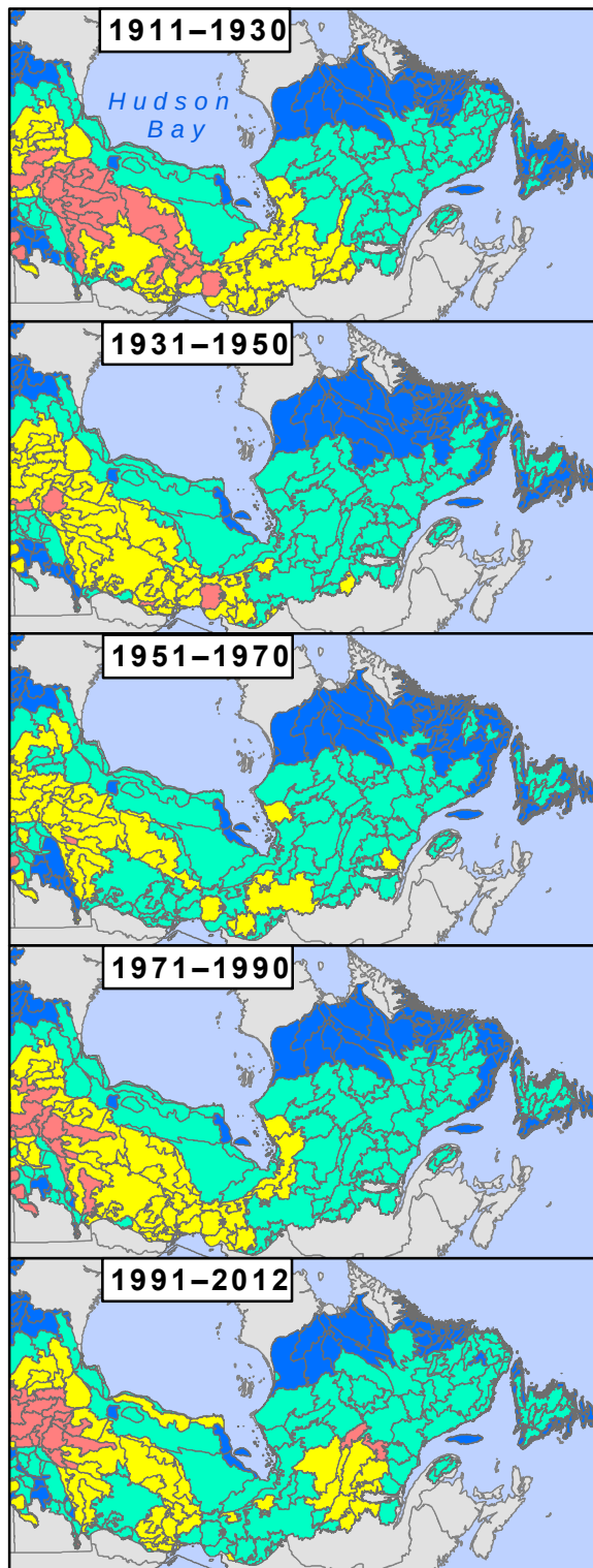
(a) Annual burn rates
