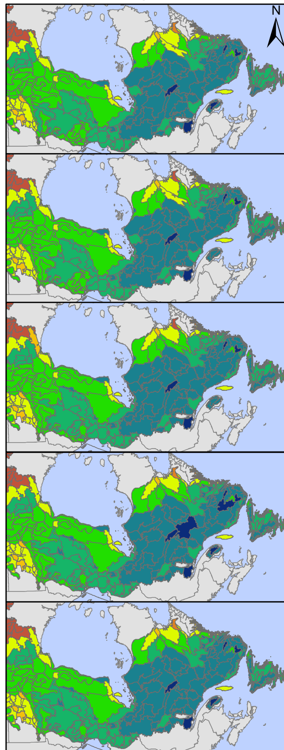
(c) Total aboveground biomass
