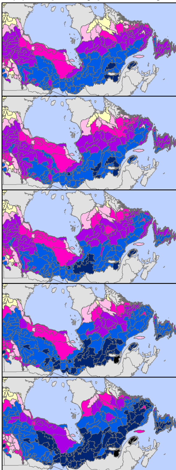
(b) Net primary productivity
