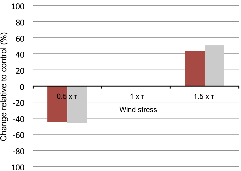
(c) Suboxic volume
