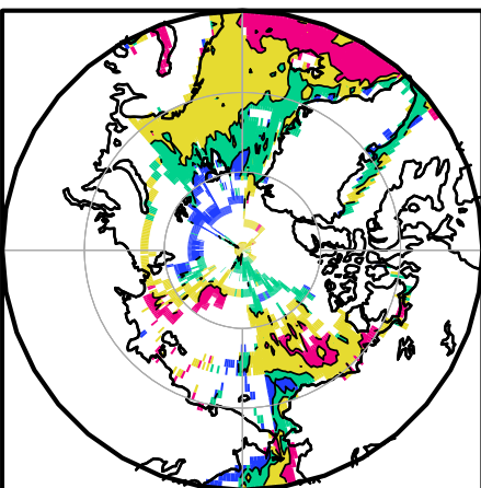
(c) p\text{CO}_{2w} (bias)
