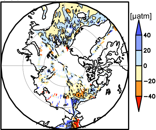
(c) p\text{CO}_{2w} (bias)
