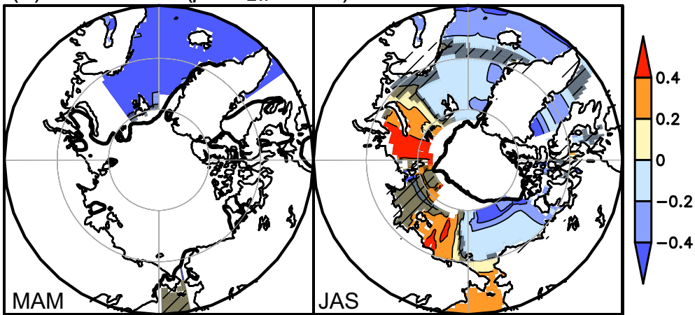
(a) Correlation ( p\text{CO}_{2w} -Chl a )
