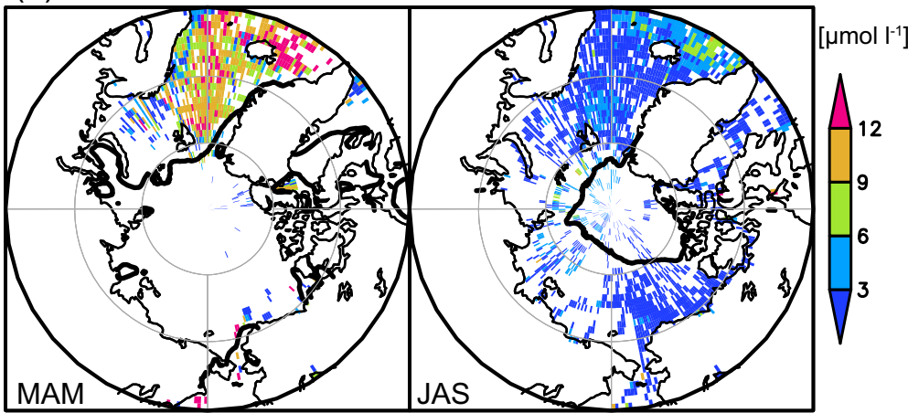
(b) Nitrate
