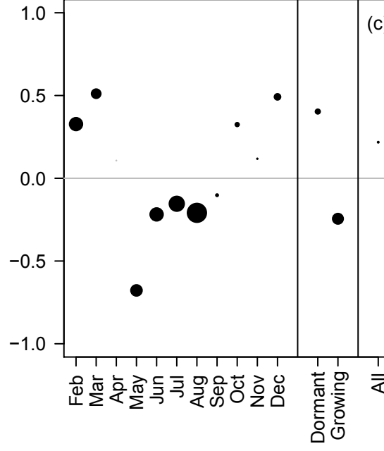
Slope SUVA-254 ~ discharge
