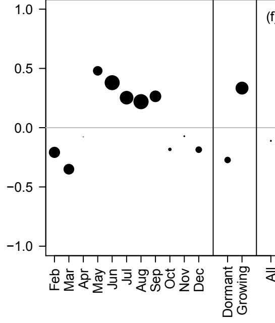
Slope viscosity ~ discharge
