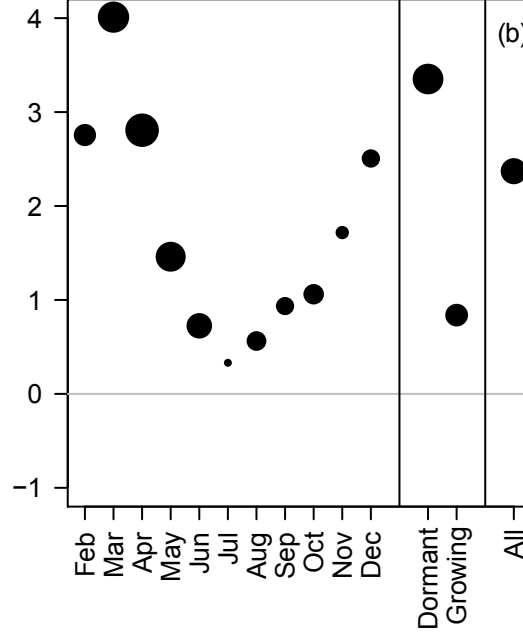
Slope SUVA-254 ~ DOC
