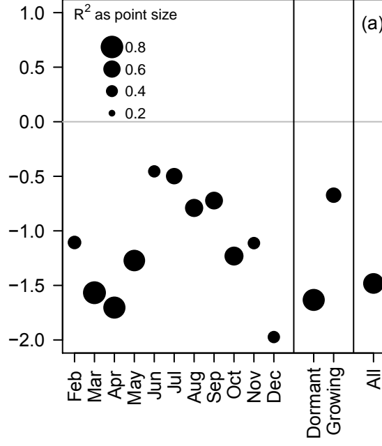
Slope SUVA-254 ~ viscosity
