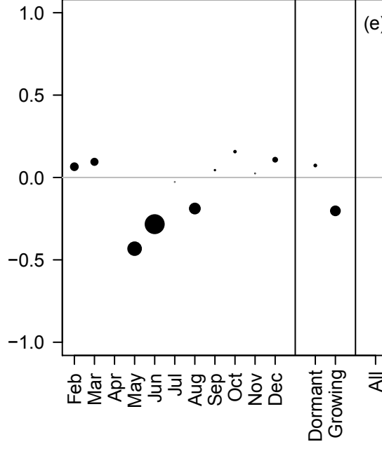
Slope DOC ~ discharge
