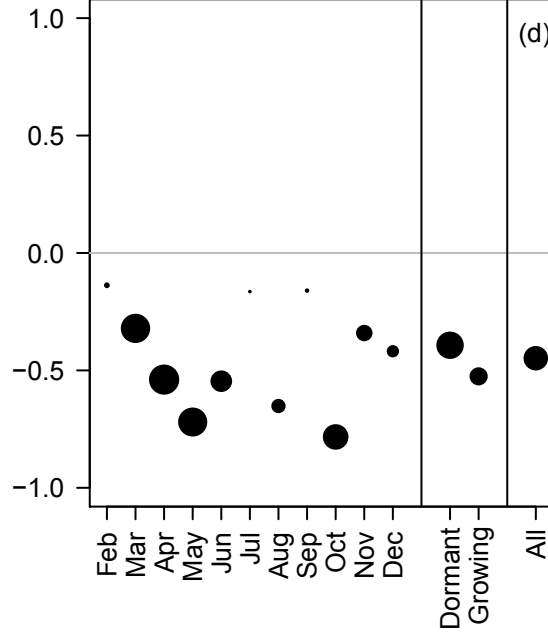
Slope DOC ~ viscosity
