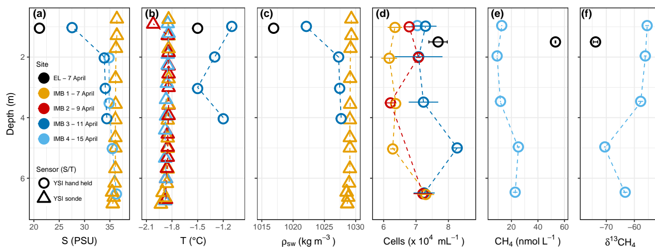
Figure 1. Water column properties during the time series near Utqiagvik. Salinity (a), temperature (b), density (c), cell abundance (d), methane concentration (e) and stable isotope ratios (f). Error bars on cell numbers (d) represent the standard deviation on two technical replicates. Salinity and temperature (a and b) were determined with a YSI hand held (circle) and YSI sonde (triangle). Salinity for the YSI hand held on 15 April was determined in the laboratory, thus in situ temperature is missing. Salinity for the YSI sonde on 9 and 15 April is missing due to freezing of the sensor. Methane data is only available for EL on 7 April and for IMB 4 on 15 April.
