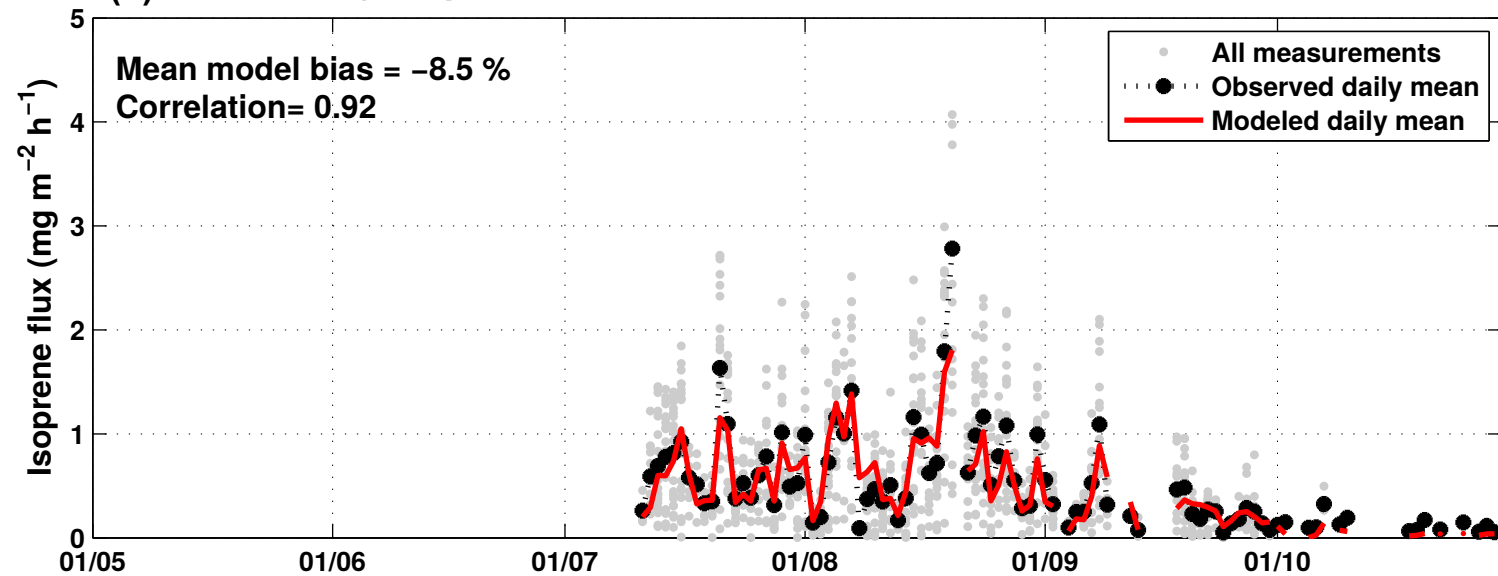
(a) Daily isoprene fluxes in 2009 at Vielsalm (50.30° N 5.99° E)
