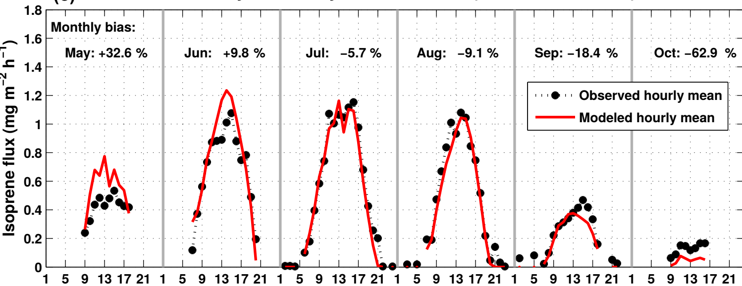
(c) Monthly diurnal cycle at Vielsalm (50.30° N 5.99° E)
