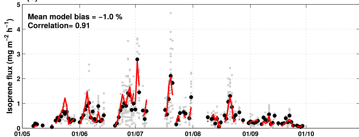
(b) Daily isoprene fluxes in 2010 at Vielsalm (50.30° N 5.99° E)
