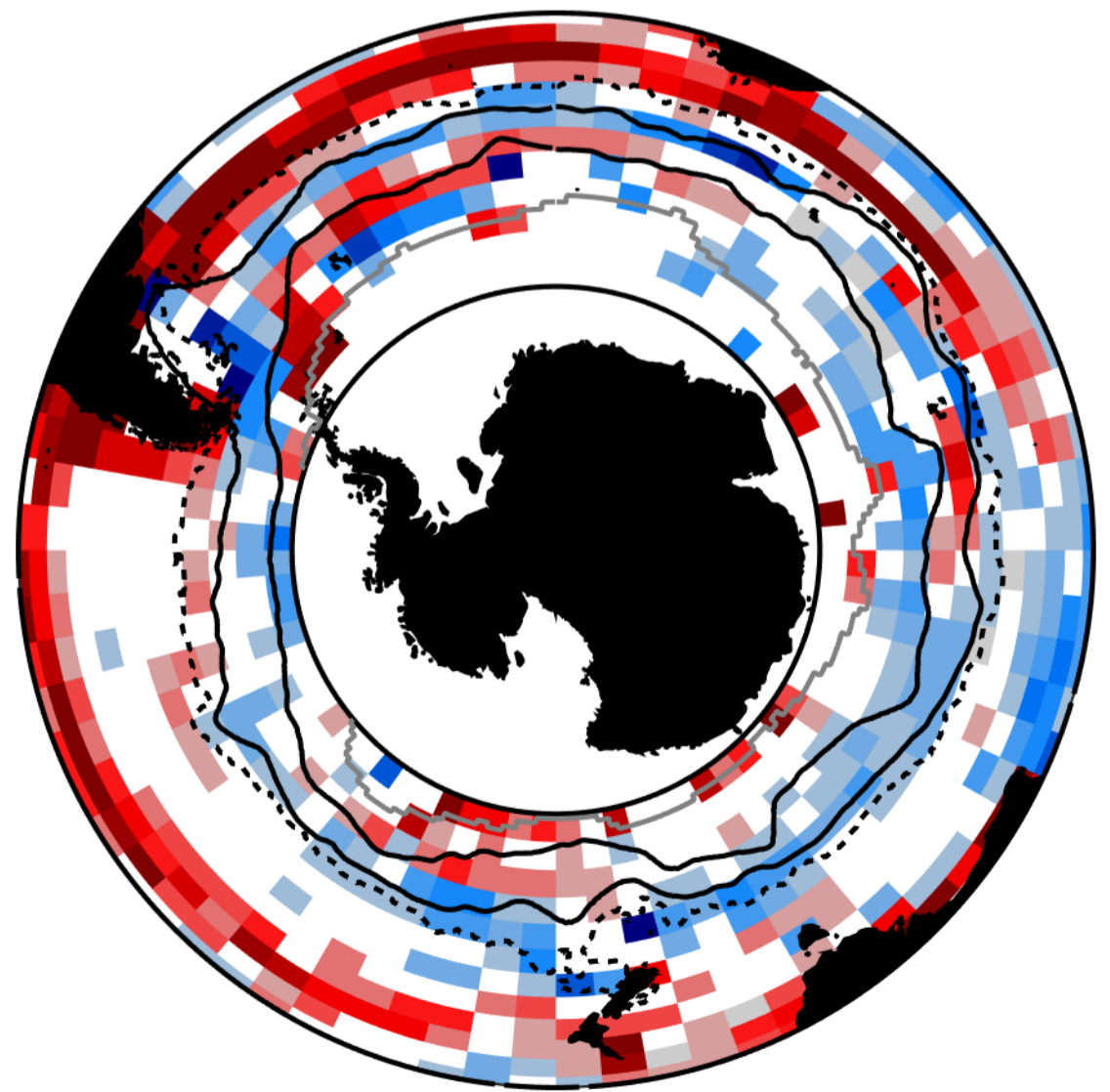
(c) \delta Chl cyclones
