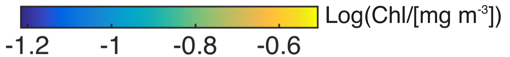
(c) \delta Chl cyclones
