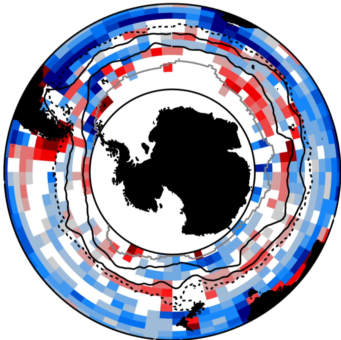
(b) \delta Chl anticyclones
