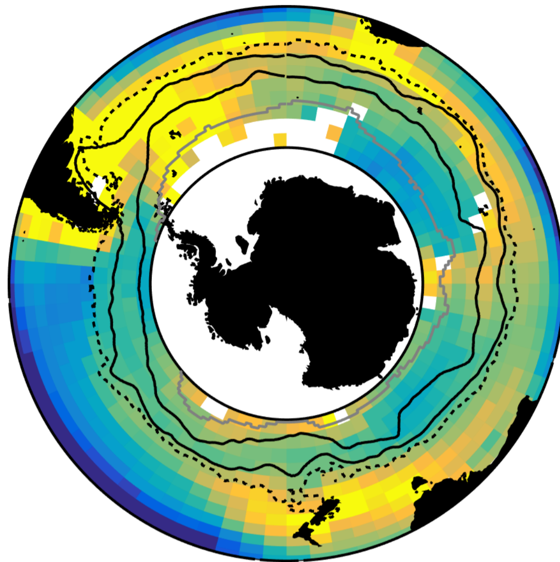
(a) Log(Chl) background
