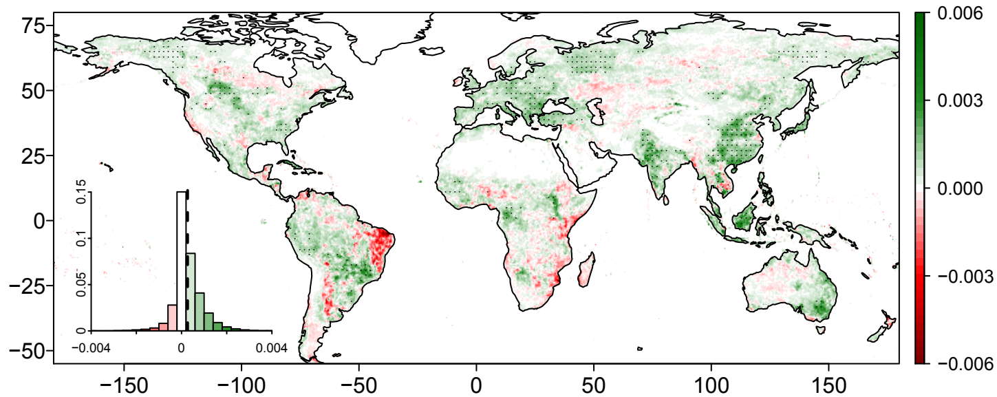
Trend of CSIF all-daily over 2001–2016
