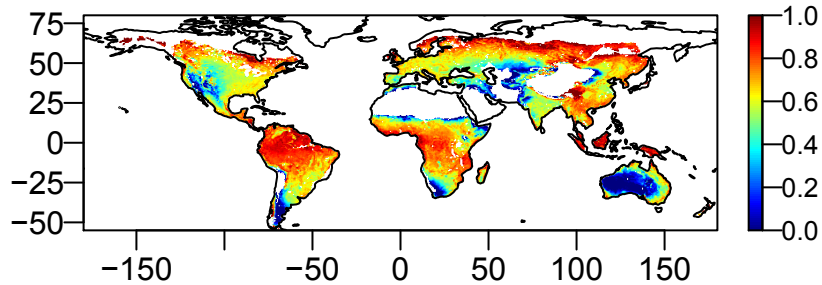
(c) Regression slope between CSIF and SIF*
