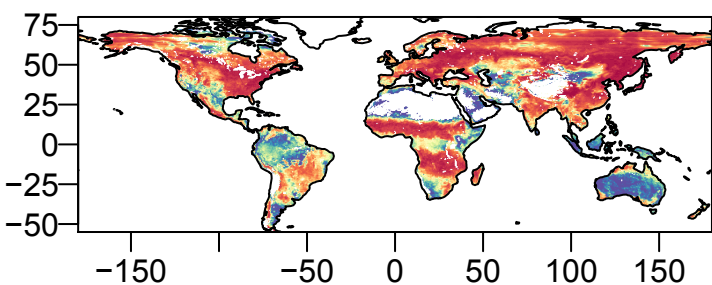
(b) R 2 between CSIF and RSIF GOME-2
