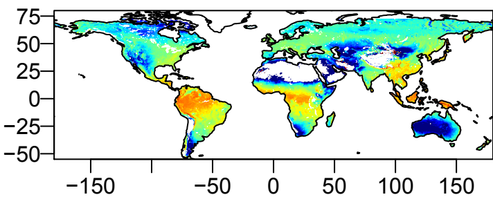
(a) Regression slope between CSIF and RSIF GOME-2
