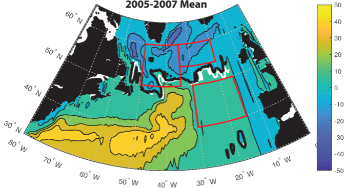
(b) Barotropic Streamfunction (Sv) 2005-2007 Mean
