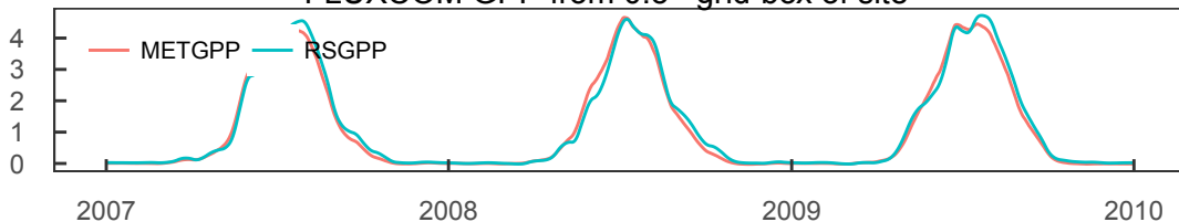
FLUXCOM GPP from 0.5° grid box of site
