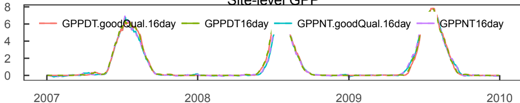
Site-level GPP
