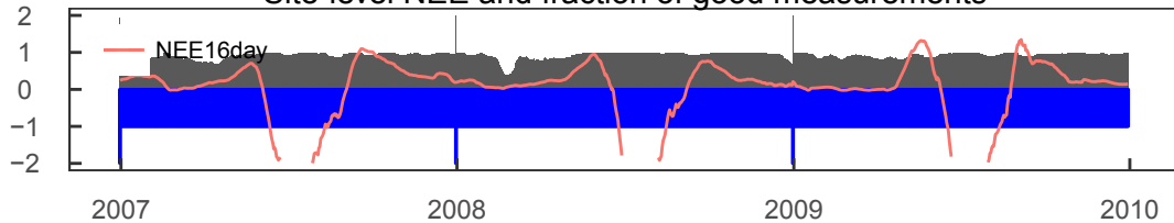
Site-level NEE and fraction of good measurements
