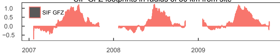
SIF GFZ footprints in radius of 30 km from site
