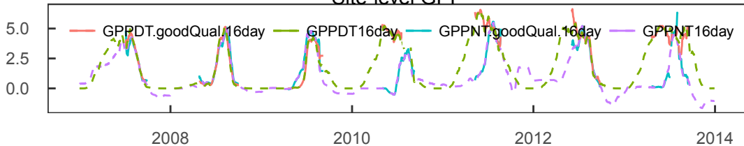
Site-level GPP
