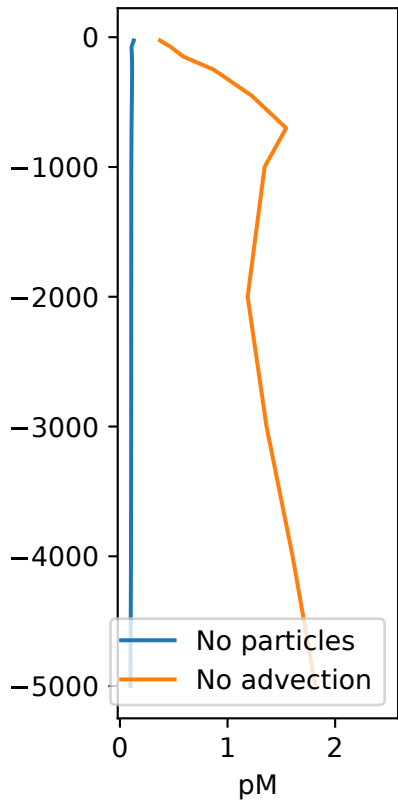
(a) Global mean
