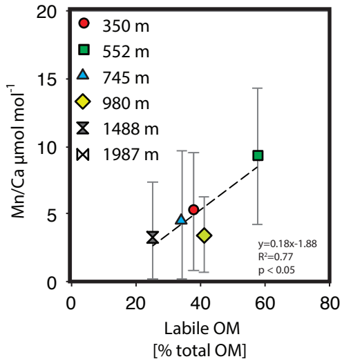
Uvigerina mediterranea
