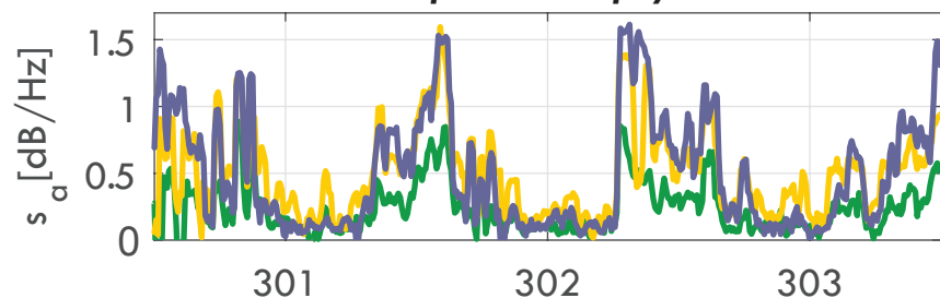
H. Wind speed
