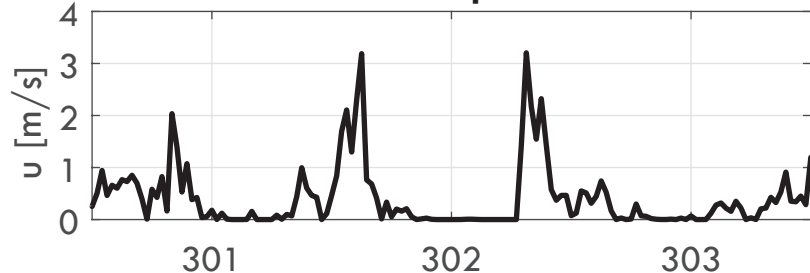
H. Wind speed
