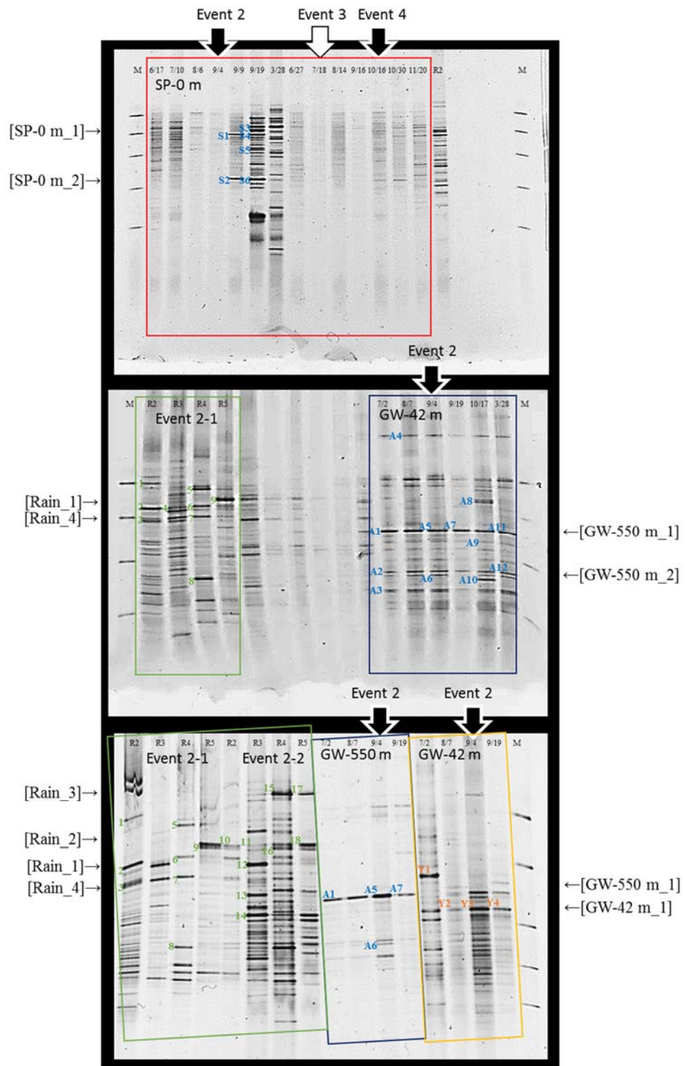
Figure S3. Bacterial community composition of groundwater (SP-0m, GW-42m and GW-550m) and rainwater (R2, R3, R4 and R5). Black and open arrows indicate the rainfall event; Event 2, Event 3 and Event 4. Black arrows particularly indicate the torrential rainfall.
