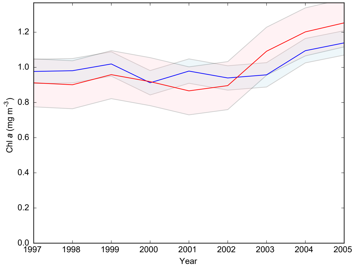
Evolution of surface Chl a
