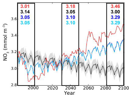
(e) Nitrate intermediate (200–600 m)
