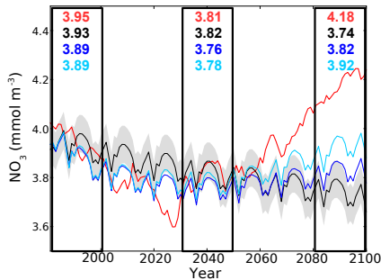
(b) Nitrate intermediate (200–600 m)
