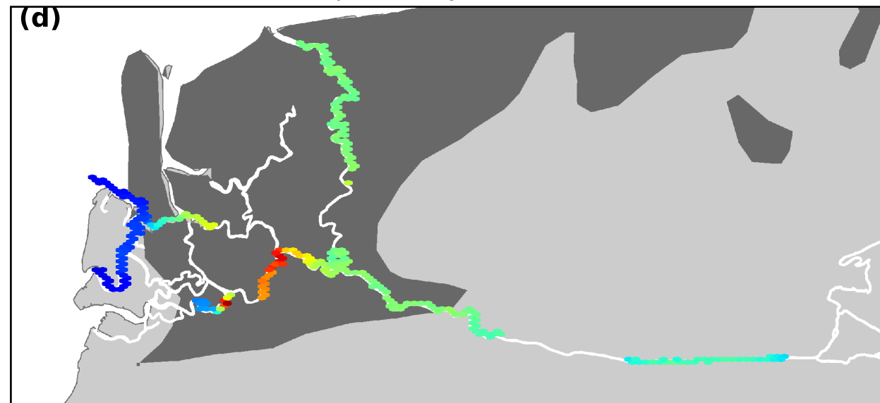
pCO 2 , dry season
