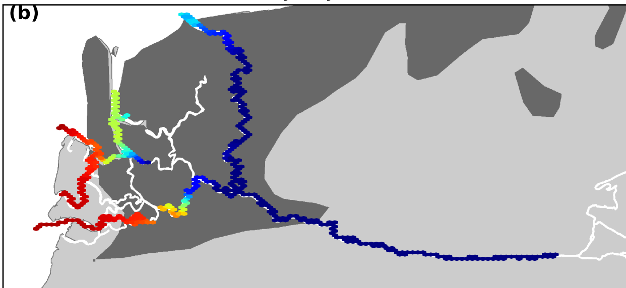
Salinity, dry season
