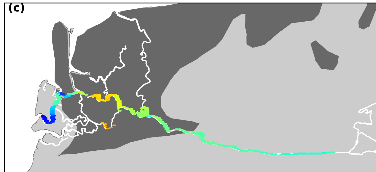
pCO 2 , wet season
