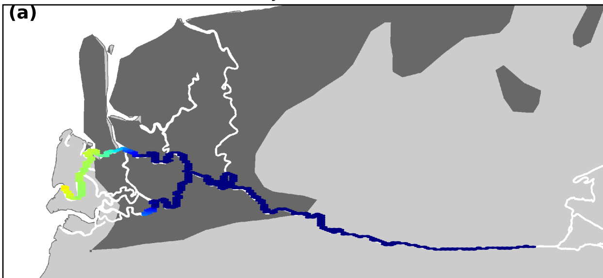
Salinity, wet season
