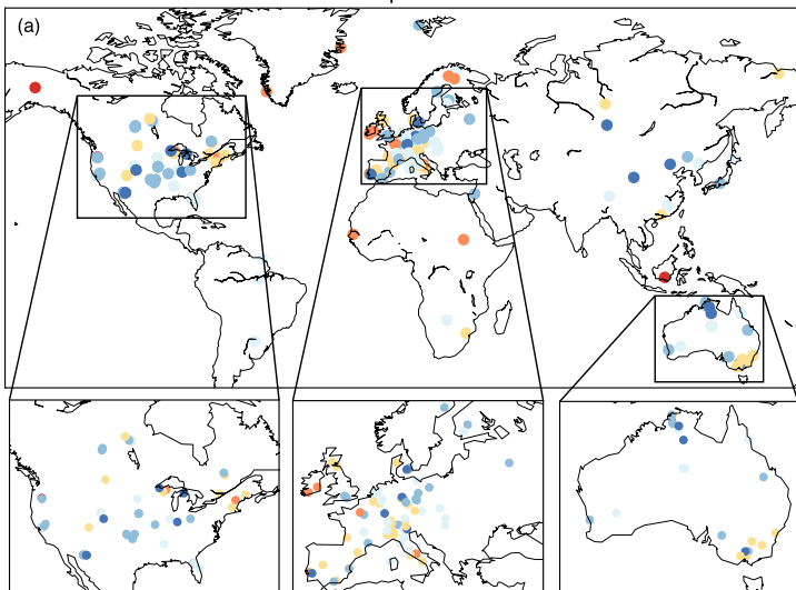
All temperatures
