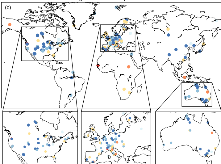
Highest 2.3 % temperatures
