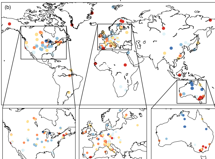
Lowest 2.3 % temperatures
